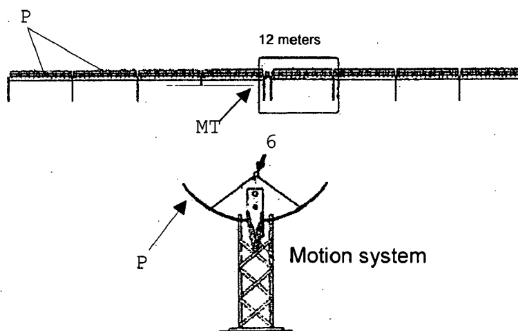
Solar collectors
