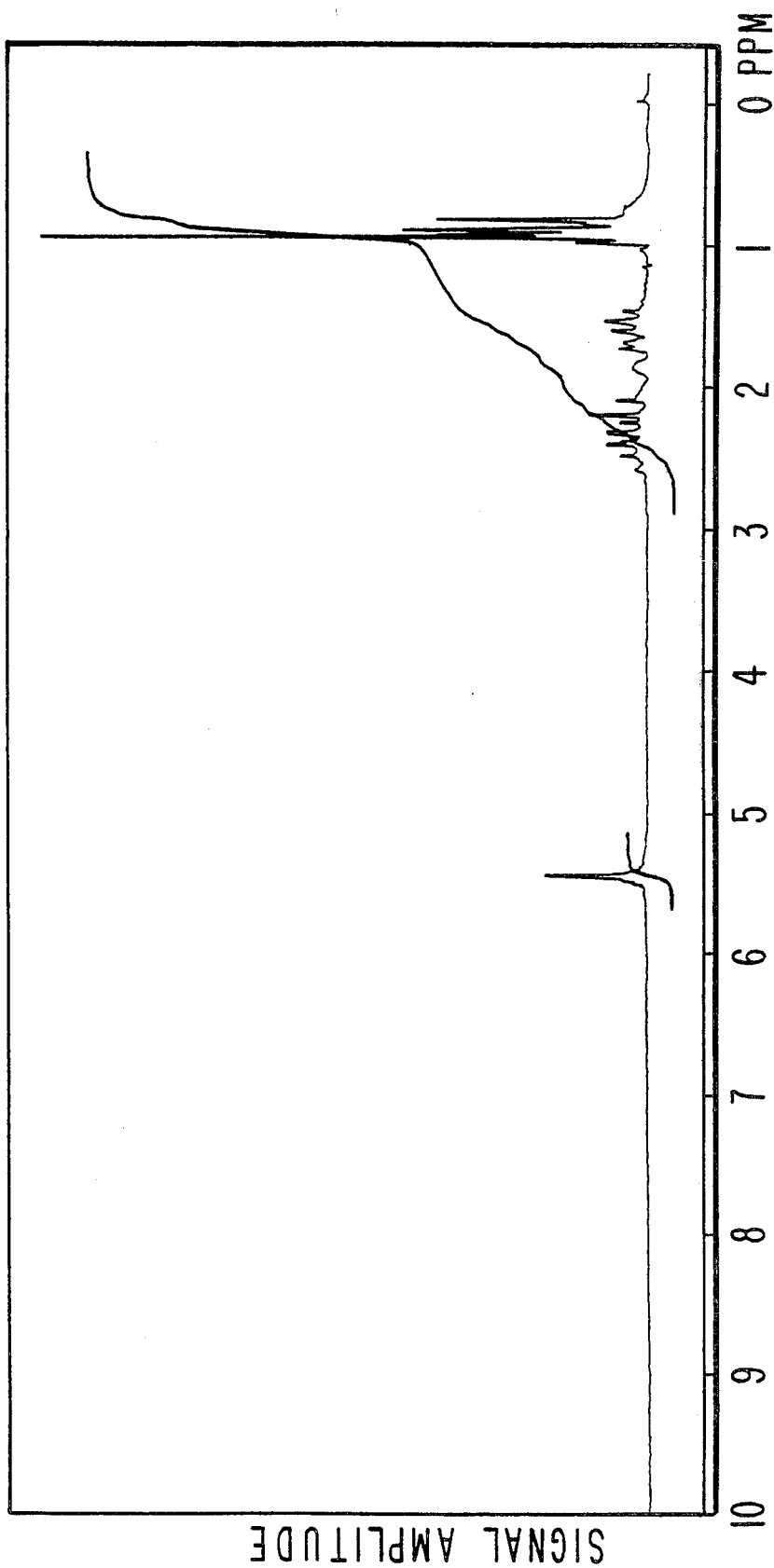
NMR SPECTRUM FOR EXAMPLE XVII
