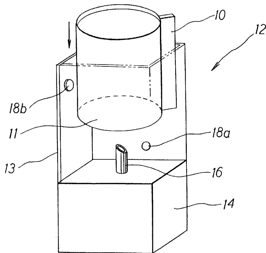
Fig. 1 (Prior Art)
