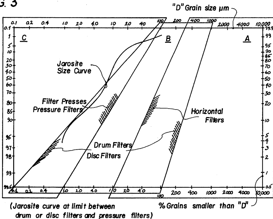
Diagram for Choice of Filter Types According to Grain Sizes
