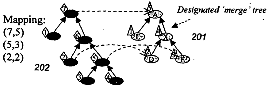
Figure: 9a Two Dataflow Trees
