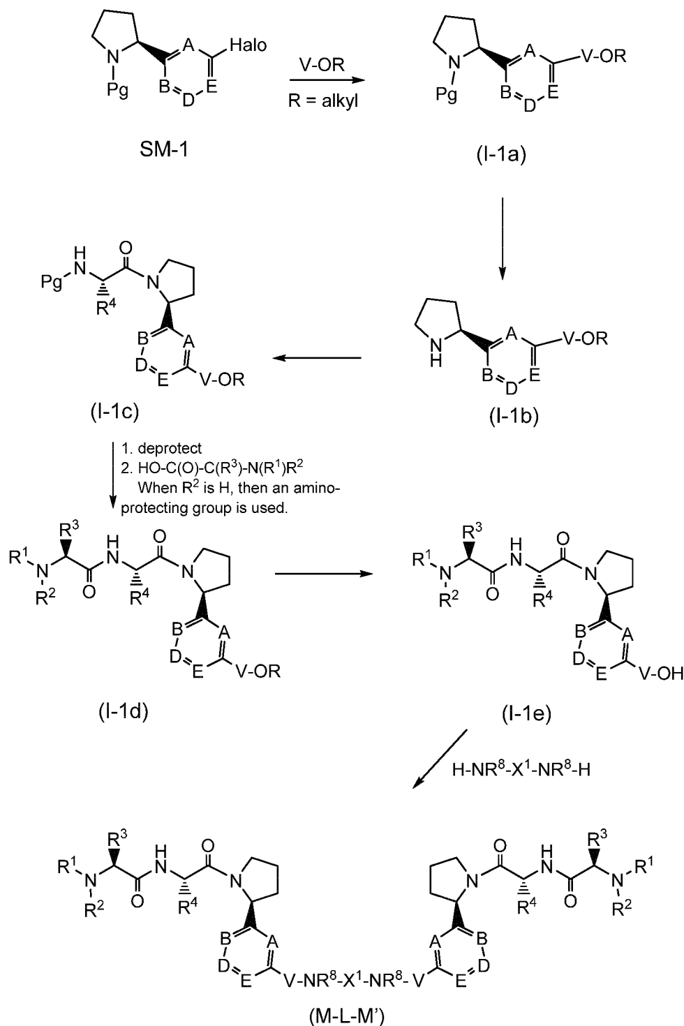
Scheme I
