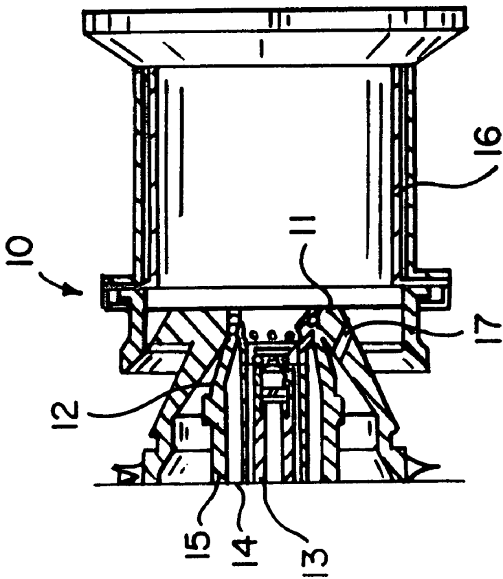
FIG. 1 PRIOR ART
