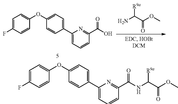
Scheme 23
