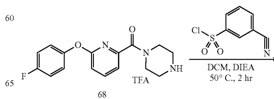
Scheme 31
