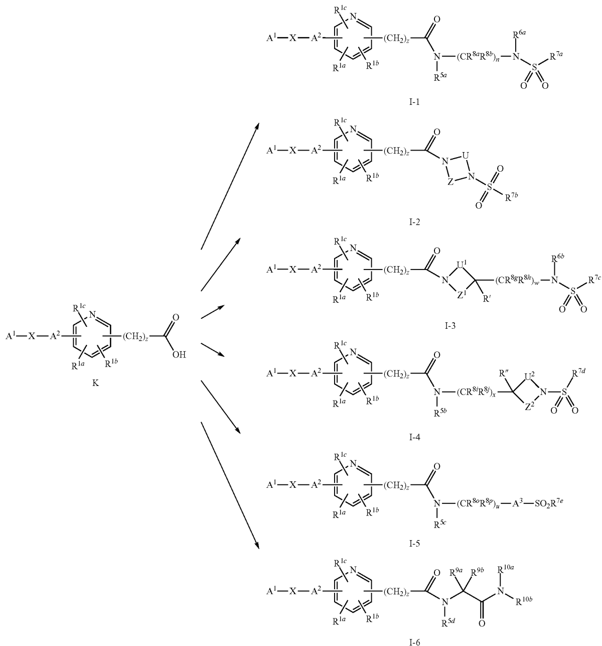
Scheme 8
