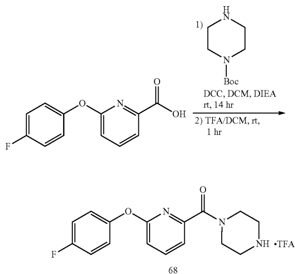
Scheme 30
