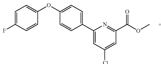
Scheme 46
