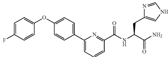
Example 18
