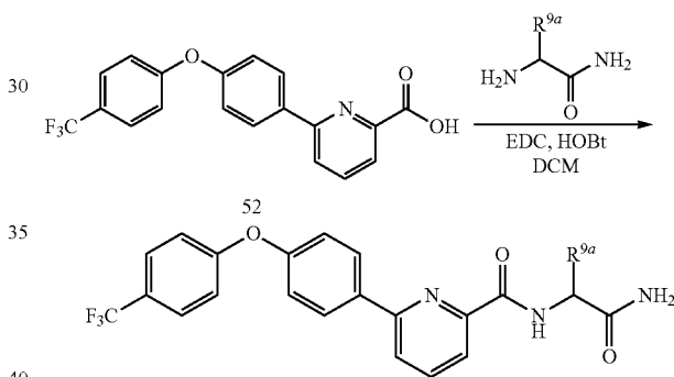
Scheme 28
