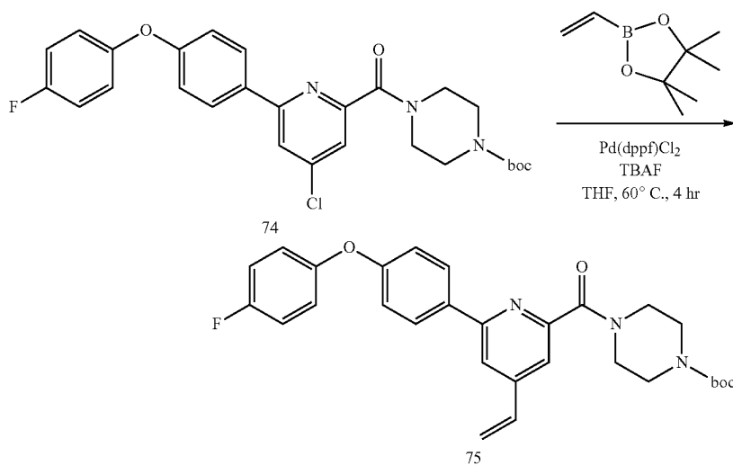
Scheme 38
