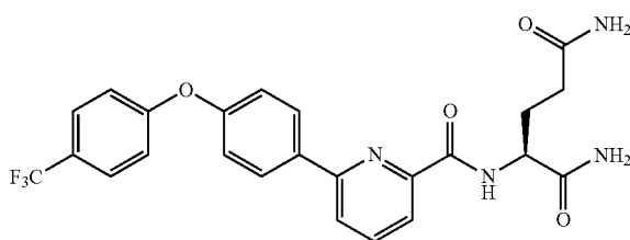
Example 20
