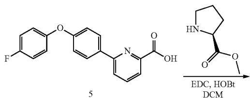
Scheme 24
