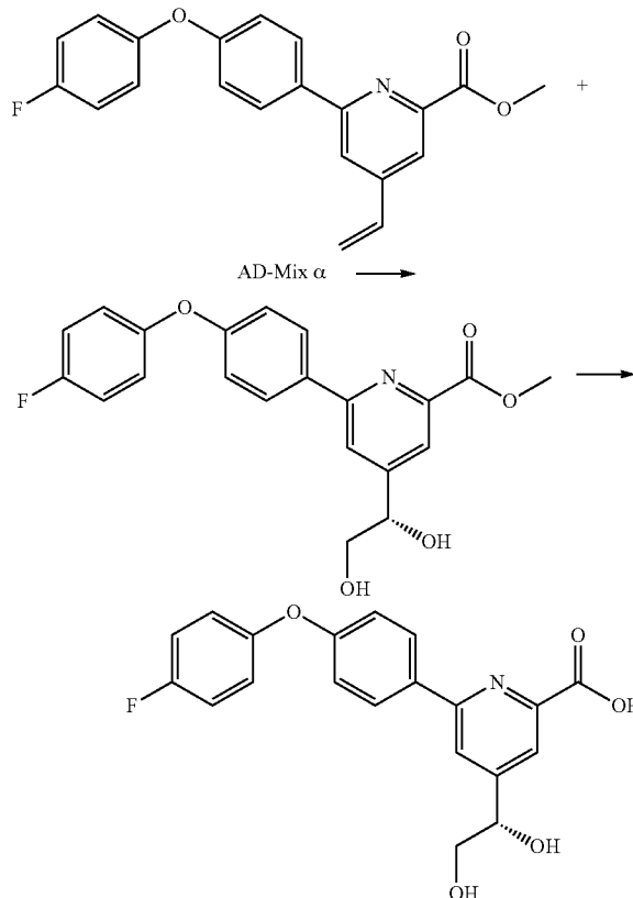
Scheme 47
