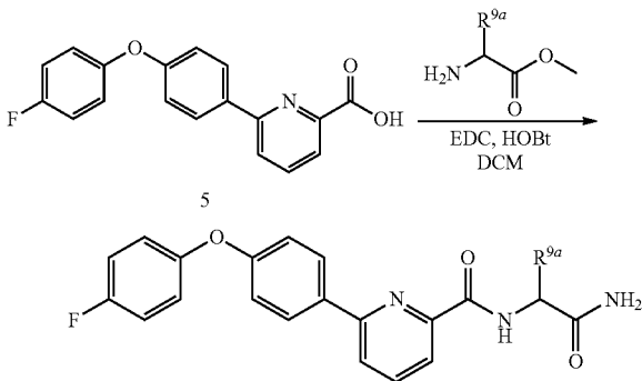
Scheme 26
