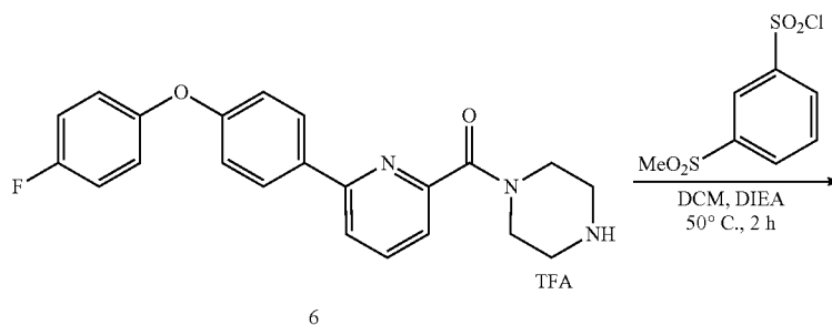
Scheme 16
