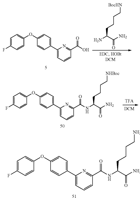
Scheme 27
