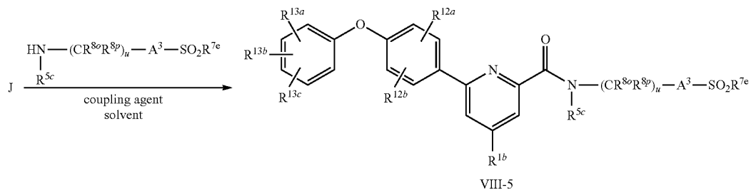
Scheme 6
