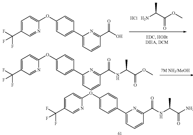
Scheme 41
