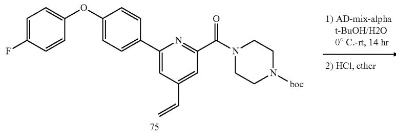
Scheme 39
