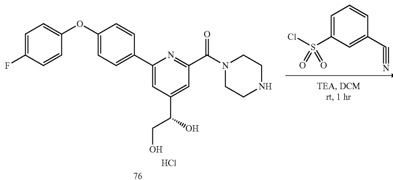
Scheme 40
