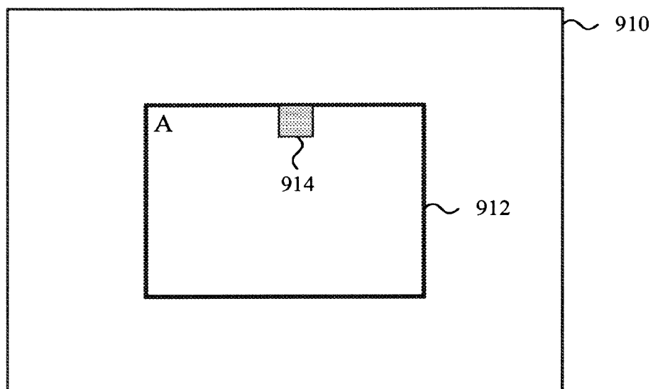
region (914) in reference frame (910), with motion constraints for tile set A (912)
