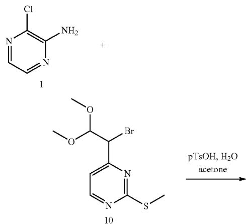
-continued Scheme 3
