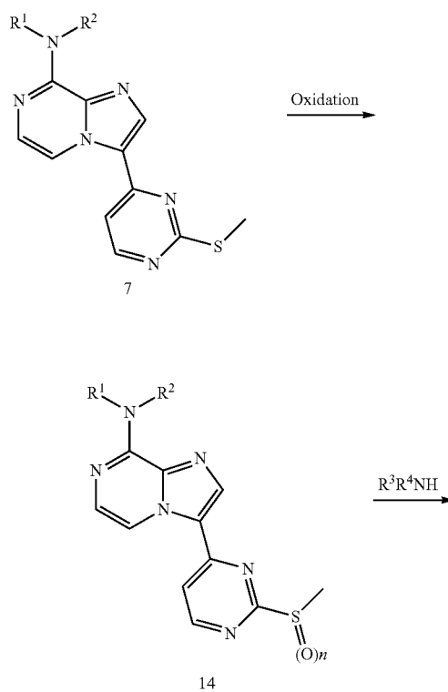
Scheme 5
