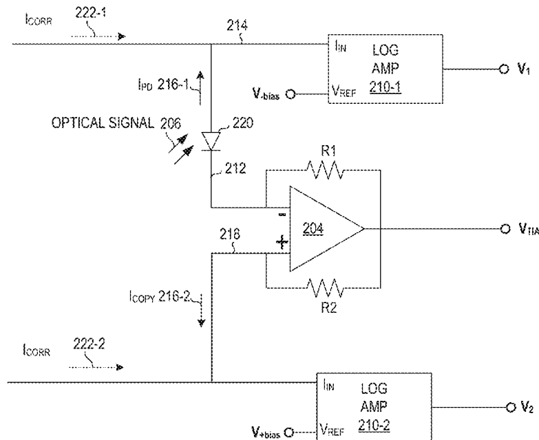
200 → TRIPLE OUTPUT PHOTODETECTOR CURRENT REPLICATOR
