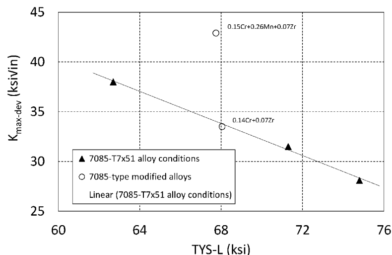
FIG. 5 - K_{\max\text{-dev}} vs. TYS-L at T/2 for ~5.3in thick plate
