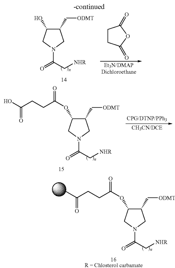
[0419] Scheme 1. Synthesis of cis-(3S,4R)-pyrrolidine diol
