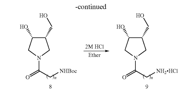
[0419] Scheme 1. Synthesis of cis-(3S,4R)-pyrrolidine diol
