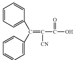
Esters of 2-Cyano-3, 3-Diphenyl-2-Propenoic Acid
