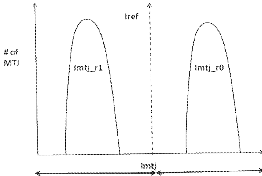
Figure 7 Non-Overlapped I_{mtj} Distribution
