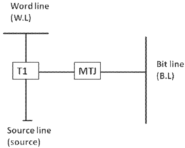
Figure 1 Magnetic Random Access Memory (MRAM) cell
