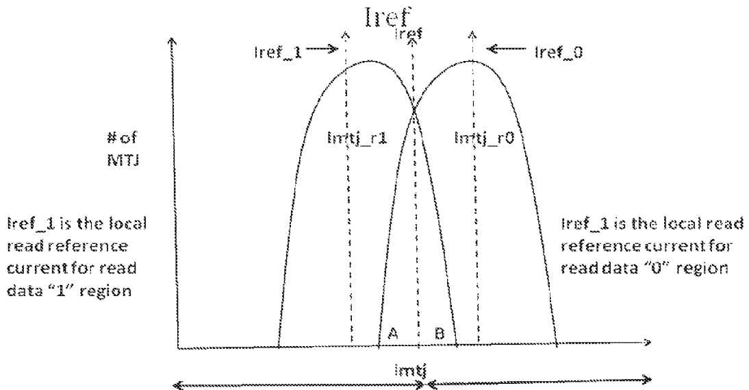
Figure 10 Overlapped I_{mtj} Distribution with additional
