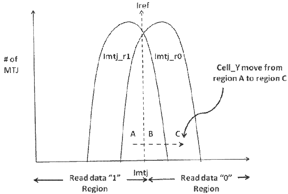
Figure 9 Overlapped I_{mtj} Distribution
