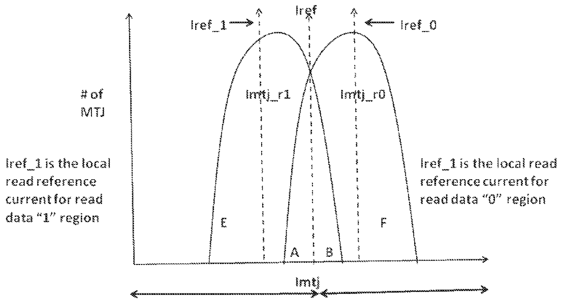
Figure 11 Additional regions as a result of additional Iref
