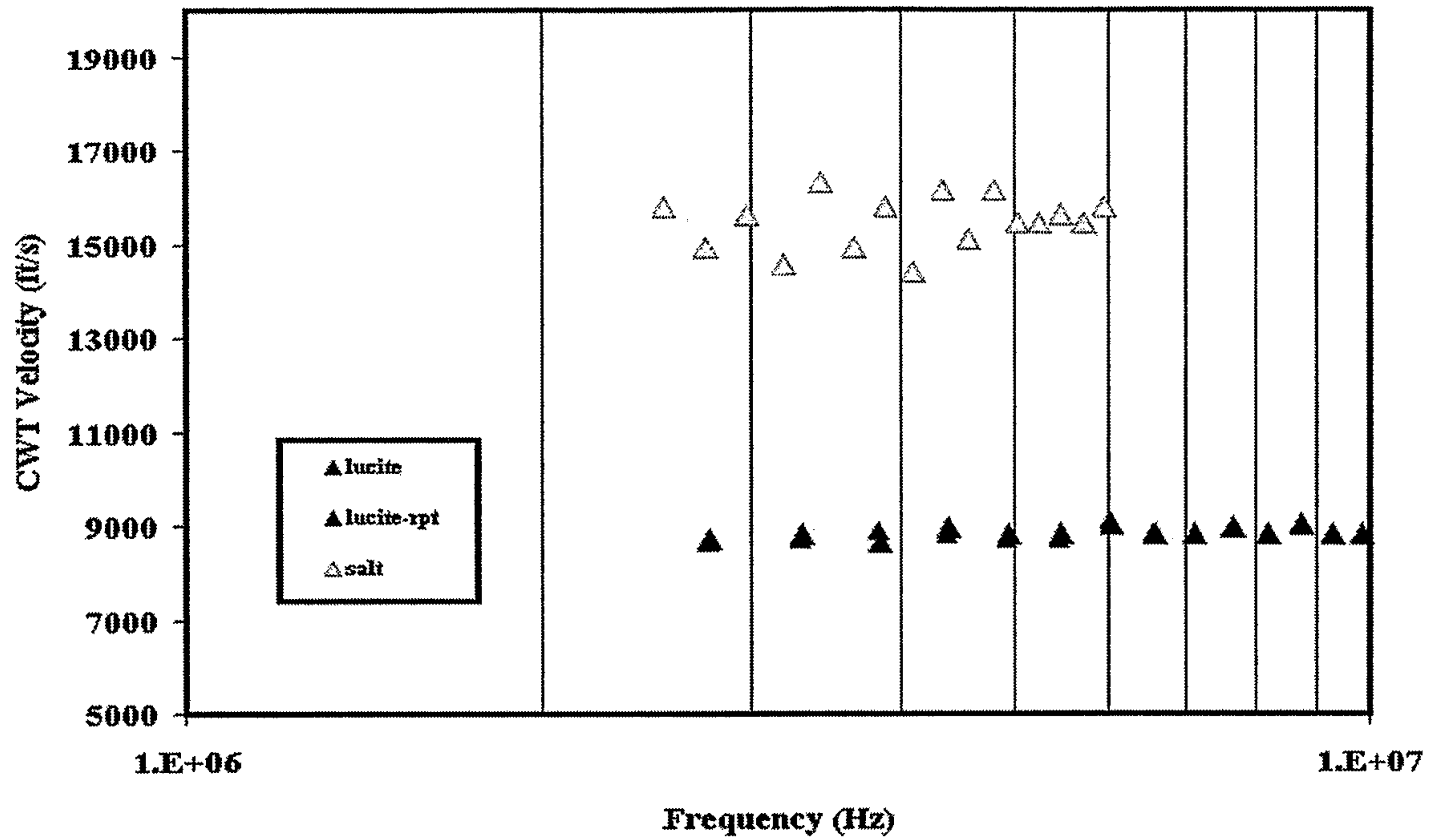
Figure 4: CWT velocity as a function of frequency for reference materials
