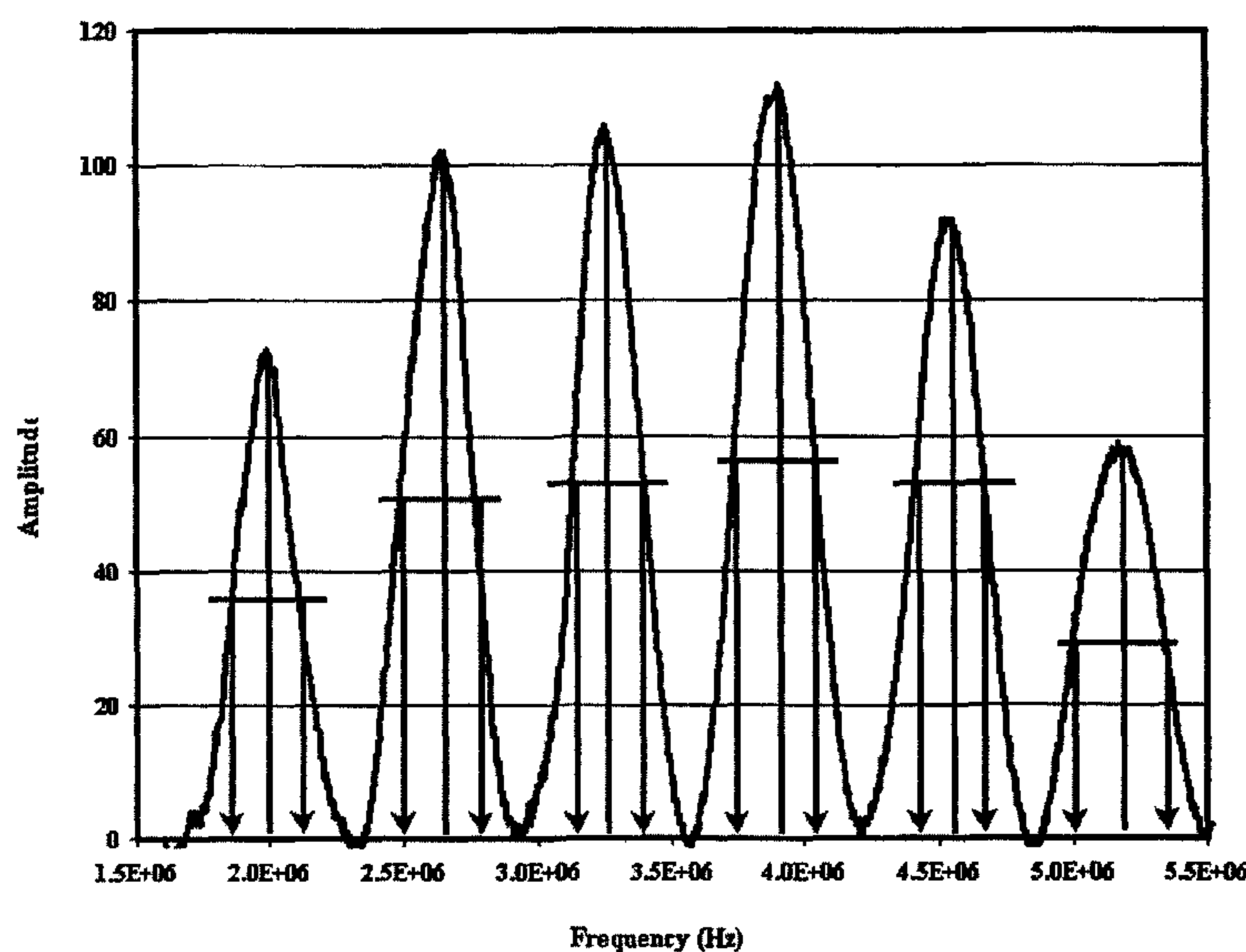
Schematic definition of attenuation calculation from CWT amplitude spectra.
