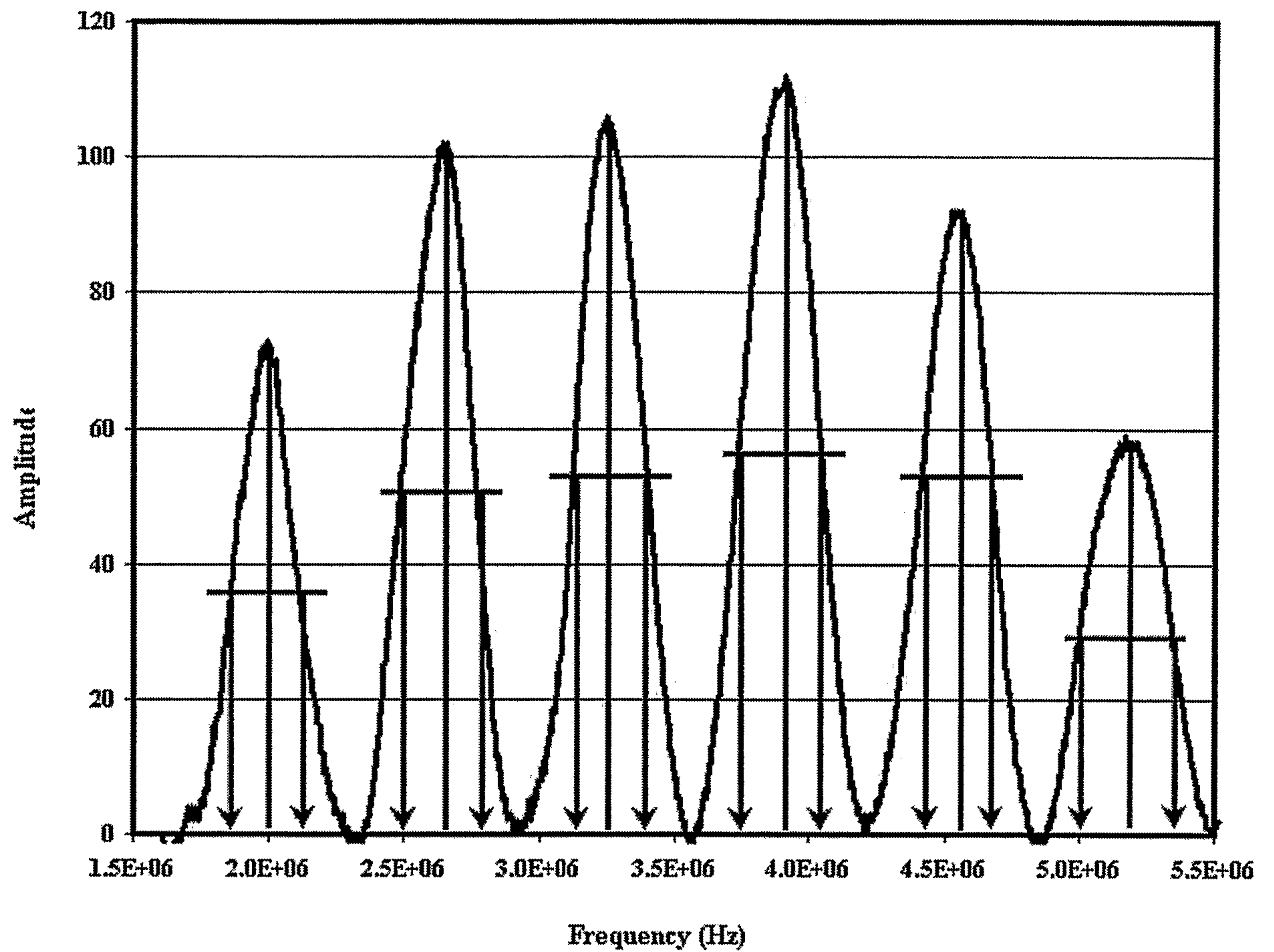
Figure 3: Schematic definition of attenuation calculation from CWT amplitude spectra.
