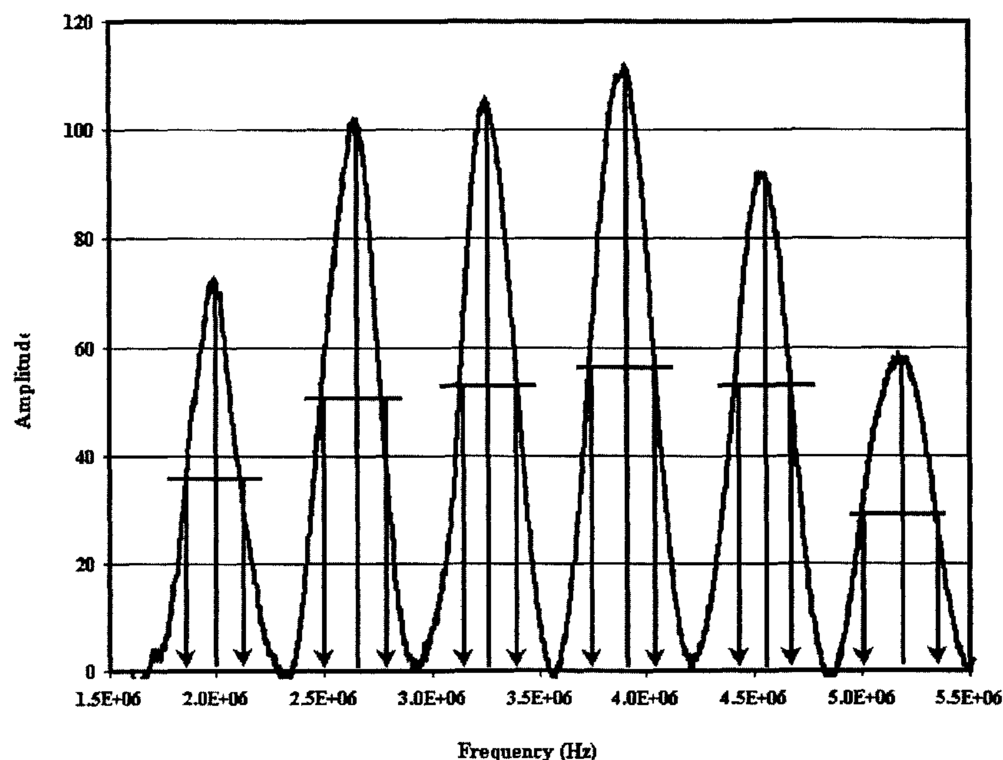
Schematic definition of attenuation calculation from CWT amplitude spectra.
