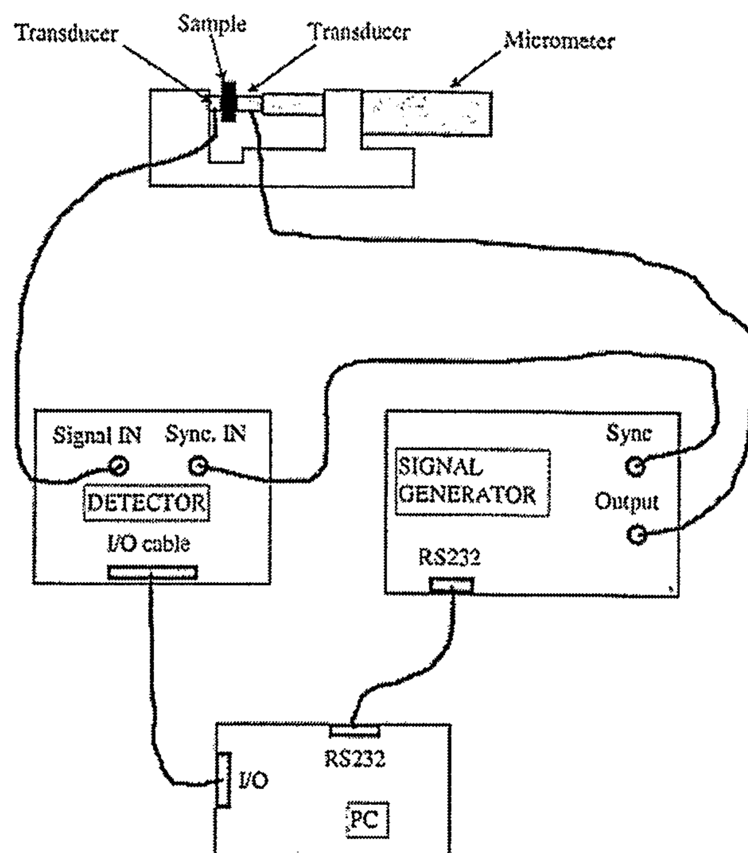
Figure 1: Experimental Set-up
