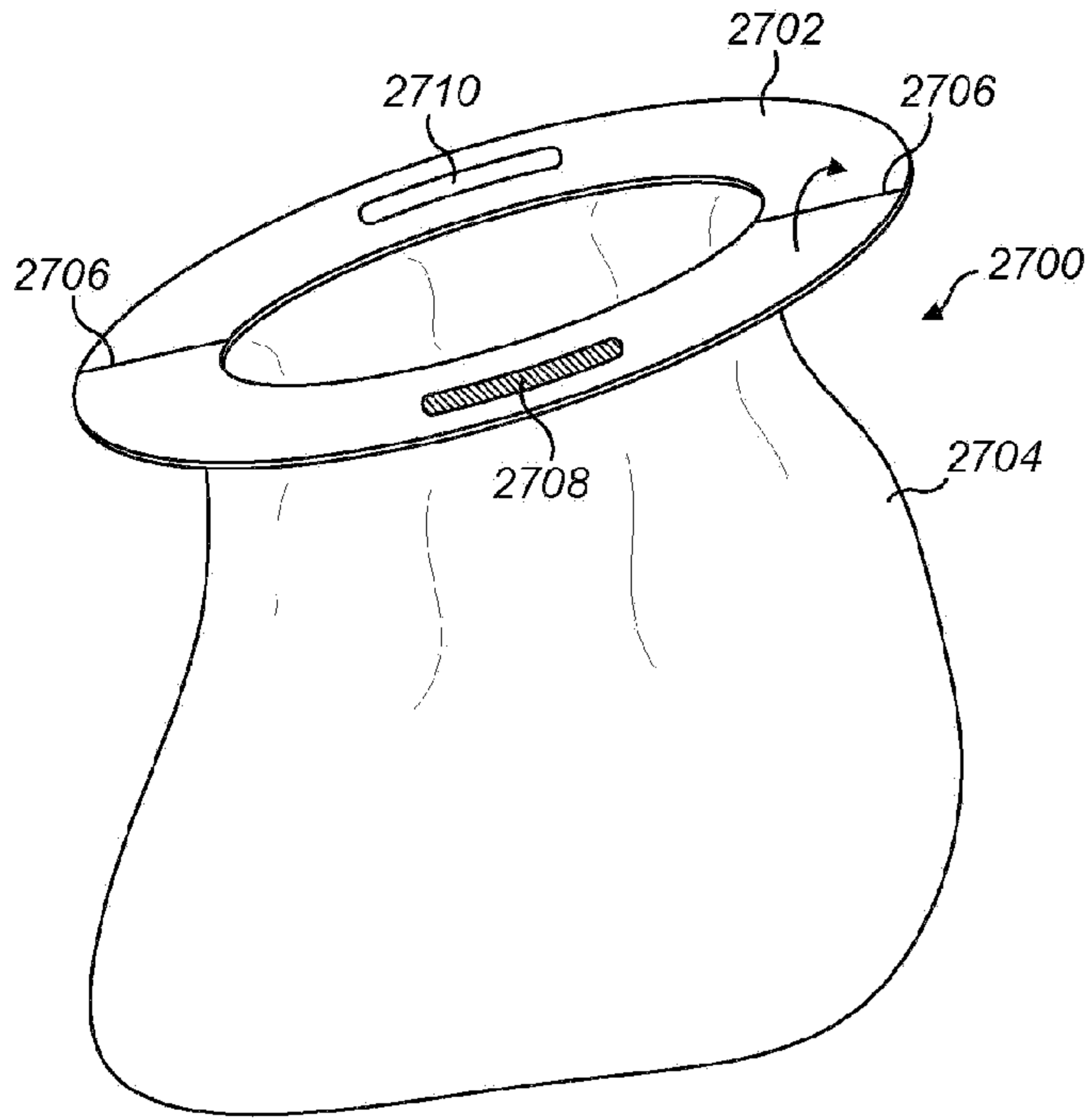
FIG. 27 (Prior Art)
