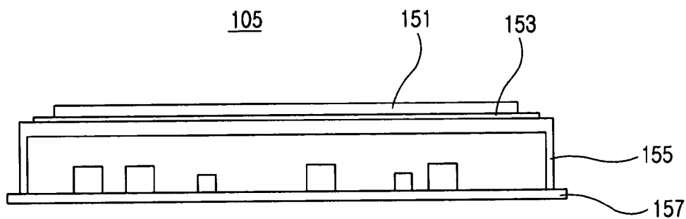
FIG.3 (PRIOR ART)
