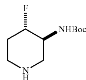
tert-Butyl-trans-4-fluoropiperidin-3-ylcarbamate
