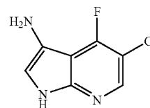
5-Chloro-4-fluoro-1H-pyrrolo[2,3-b]pyridine-3-amine
