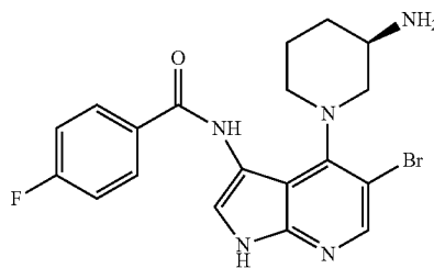
(R)-N-(4-(3-Aminopiperidin-1-yl)-5-bromo-1H-pyrrolo[2,3-b]pyridin-3-yl)-4-fluorobenzamide
