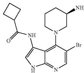
(R)-N-(4-(3-Aminopiperidin-1-yl)-5-bromo-1H-pyrrolo[2,3-b]pyridin-3-yl)cyclobutanecarboxamide
