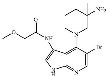
N-(4-(3-Amino-3-methylpiperidin-1-yl)-5-bromo-1H-pyrrolo[2,3-b]pyridin-3-yl)-2-methoxyacetamide
