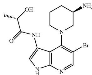
(S)-N-(4-((R)-3-Aminopiperidin-1-yl)-5-bromo-1H-pyrrolo[2,3-b]pyridin-3-yl)-2-hydroxypropanamide
