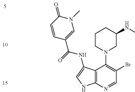
(R)-N-(5-Bromo-4-(3-(methylamino)piperidin-1-yl)-1-methyl-6-oxo-1,6-dihydropyridine-3-carboxamide)-1H-pyrrolo[2,3-b]pyridin-3-yl-1-methyl-6-oxo-1,6-dihydropyridine-3-carboxamide
