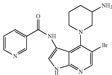
N-(4-(3-Aminopiperidin-1-yl)-5-bromo-1H-pyrrolo[2,3-b]pyridin-3-yl)nicotinamide
