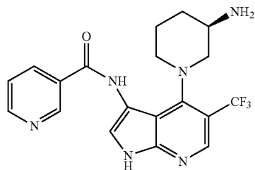
(R)-N-(4-(3-Aminopiperidin-1-yl)-5-(trifluoromethyl)-1H-pyrrolo[2,3-b]pyridin-3-yl)nicotinamide
