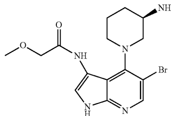
(R)-N-(4-(3-Aminopiperidin-1-yl)-5-bromo-1H-pyrrolo[2,3-b]pyridin-3-yl)-2-methoxyacetamide
