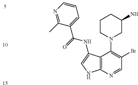
(R)-N-(4-(3-Aminopiperidin-1-yl)-5-bromo-1H-pyrrolo[2,3-b]pyridin-3-yl)-2-methylnicotinamide
