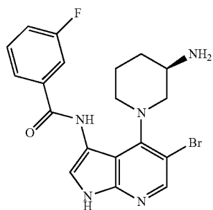
(R)-N-(4-(3-Aminopiperidin-1-yl)-5-bromo-1H-pyrrolo[2,3-b]pyridin-3-yl)-3-fluorobenzamide
