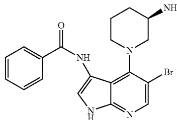
(R)-N-(4-(3-Aminopiperidin-1-yl)-5-bromo-1H-pyrrolo[2,3-b]pyridin-3-yl)benzamide
