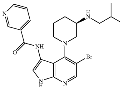
(R)-N-(5-Bromo-4-(3-(isobutylamino)piperidin-1-yl)-1H-pyrrolo[2,3-b]pyridin-3-yl)nicotinamide
