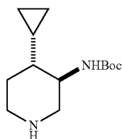
tert-Butyl-trans-4-cyclopropylpiperidin-3-ylcarbamate
