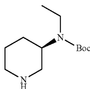
(R)-tert-Butyl ethyl (piperidin-3-yl)carbamate
