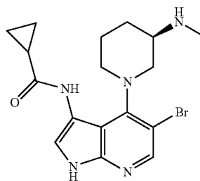
(R)-N-(5-Bromo-4-(3-(methylamino)piperidin-1-yl)-1H-pyrrolo[2,3-b]pyridin-3-yl)cyclopropanecarboxamide
