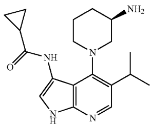
(R)-N-(4-(3-Aminopiperidin-1-yl)-5-isopropyl-1H-pyrrolo[2,3-b]pyridin-3-yl)cyclopropanecarboxamide
