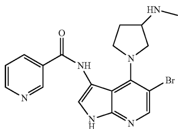
N-(5-Bromo-4-(3-(methylamino)pyrrolidin-1-yl)-1H-pyrrolo[2,3-b]pyridin-3-yl)nicotinamide
