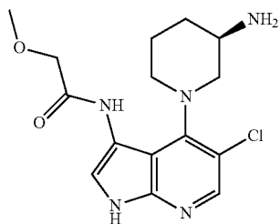
(R)-N-(4-(3-Aminopiperidin-1-yl)-5-chloro-1H-pyrrolo[2,3-b]pyridin-3-yl)-2-methoxyacetamide
