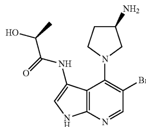
(S)-N-(4-((R)-3-Aminopyrrolidin-1-yl)-5-bromo-1H-pyrrolo[2,3-b]pyridin-3-yl)-2-hydroxypropanamide
