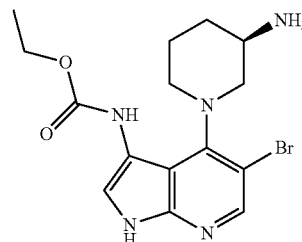
(R)-Ethyl 4-(3-aminopiperidin-1-yl)-5-bromo-1H-pyrrolo[2,3-b]pyridin-3-yl carbamate
