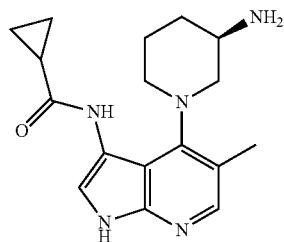
(R)-N-(4-(3-Aminopiperidin-1-yl)-5-methyl-1H-pyrrolo[2,3-b]pyridin-3-yl)cyclopropanecarboxamide
