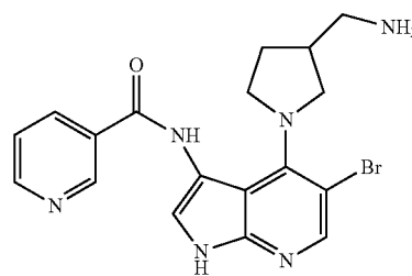
N-(4-(3-(Aminomethyl)pyrrolidin-1-yl)-5-bromo-1H-pyrrolo[2,3-b]pyridin-3-yl)nicotinamide
