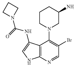
(R)-N-(4-(3-aminopiperidin-1-yl)-5-bromo-1H-pyrrolo[2,3-b]pyridin-3-yl)azetidine-1-carboxamide
