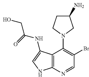
(R)-N-(4-(3-Aminopyrrolidin-1-yl)-5-bromo-1H-pyrrolo[2,3-b]pyridin-3-yl)-2-hydroxypropanamide
