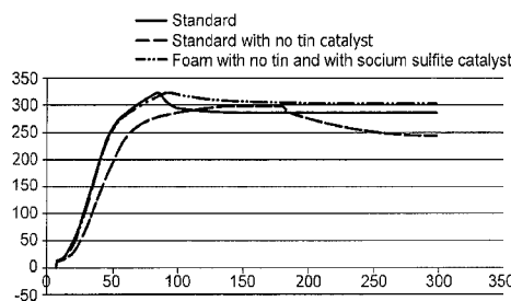
Foam 1 using standard Dabco®T-9 catalyst, Foam 2 without Dabco®T-9 catalyst showing foam collapse and Foam 3 without Dabco®T-9 catalyst and with 0.16 pphp active sodium sulfite salt (1.06 pphp of sodium sulfite solution in water).
