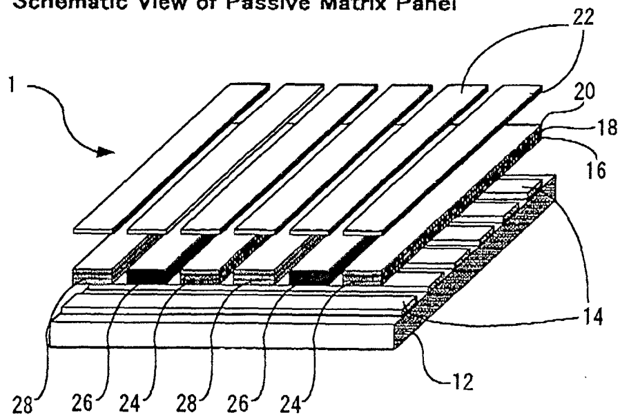
Schematic View of Passive Matrix Panel
