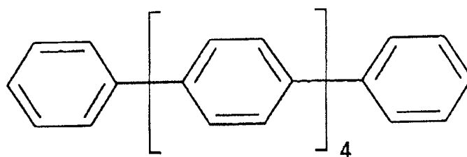
P-sexiphenyl
