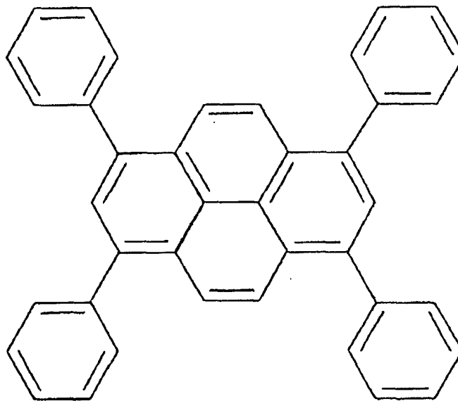
1,3,6,8-tetraphenylpyrene
