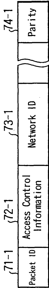
FIG. 7A Example of Structure of Header Information of Access Control Packet
