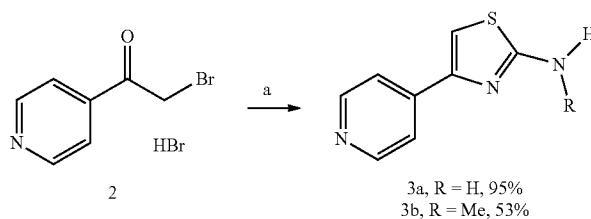
Scheme 1. First approach to the synthesis of ureas 1, 6, and 8
