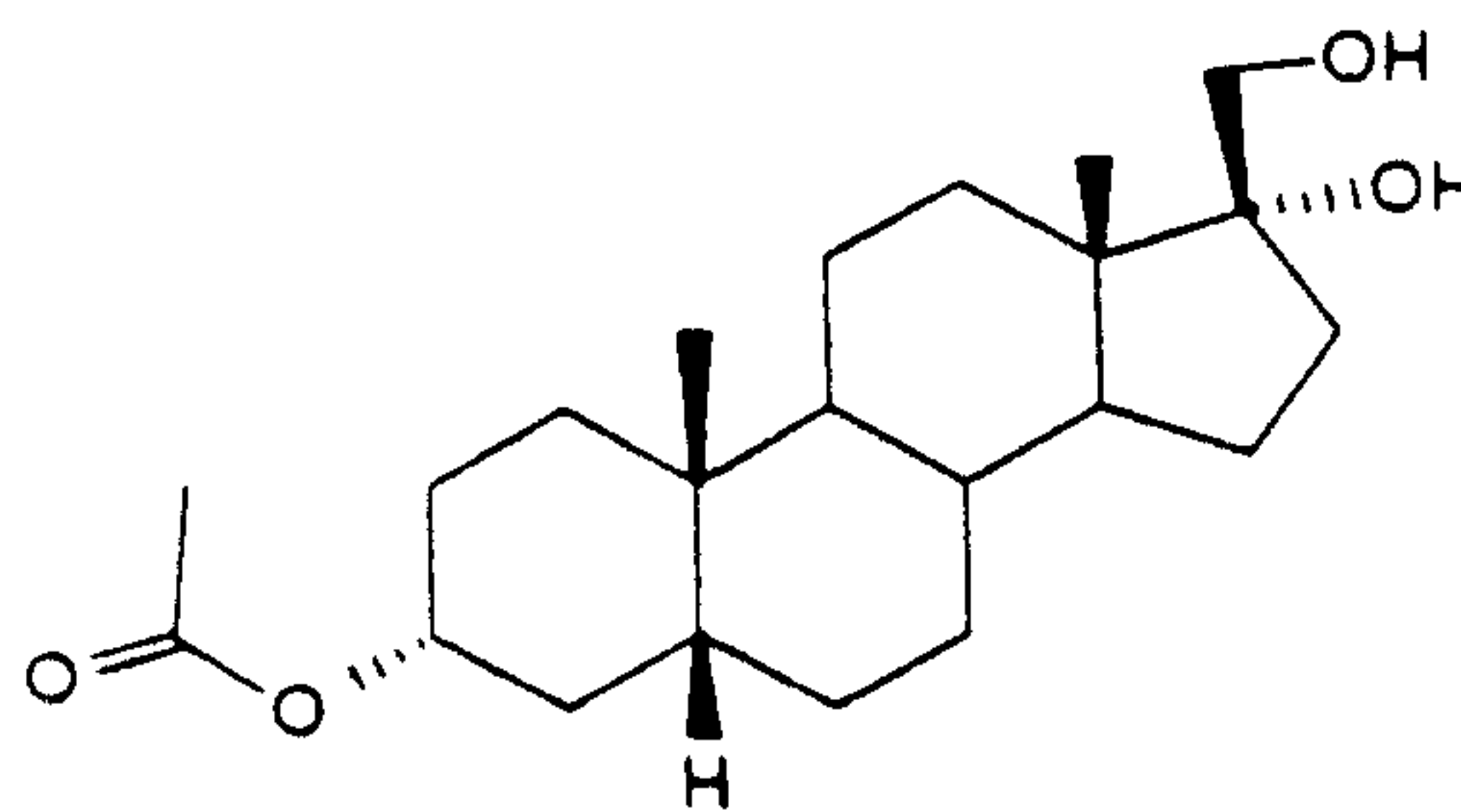
21-NOR-5 \beta -PREGNAN-17 \alpha ,20-DIOL- 3-ACETATE
