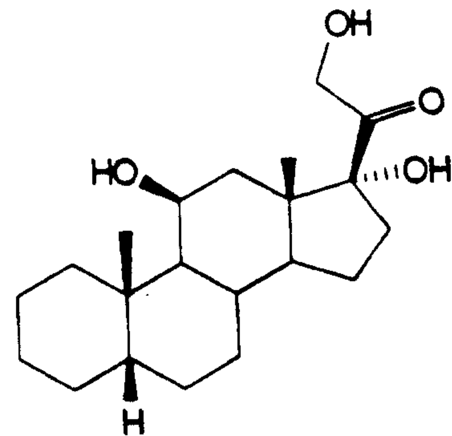
5 \beta -PREGNAN-11 \beta ,17 \alpha ,21-TRIOL-20-ONE
