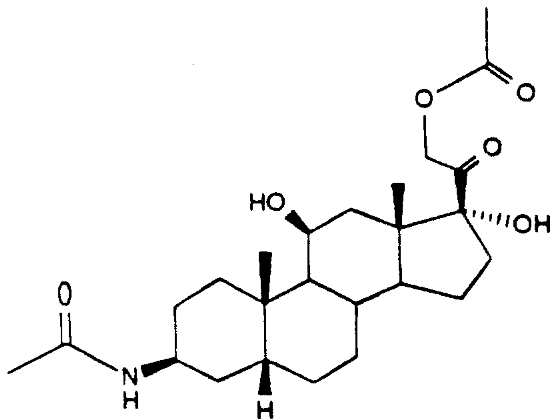
5 3 \beta -ACETAMIDO-5 \beta - PREGNAN-11 \beta ,17 \alpha , 21-TRIOL- 20-ONE-21-ACETATE
