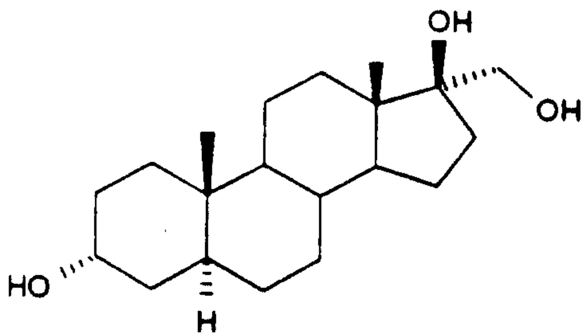
21-NOR-5 \alpha -PREGNAN-3 \alpha ,17 \beta ,20-TRIOL
