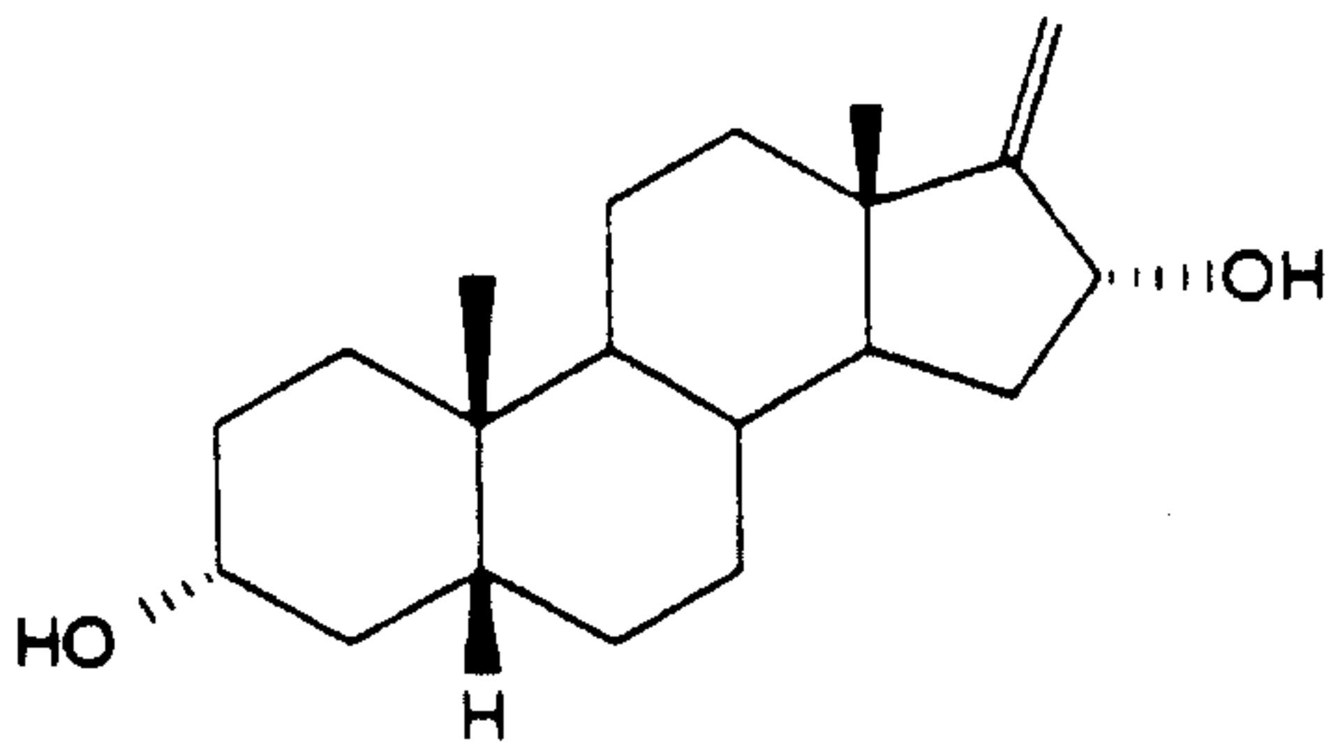
21-NOR-5 \beta -PREGN-17(20)-EN-3 \alpha ,16-DIOL
