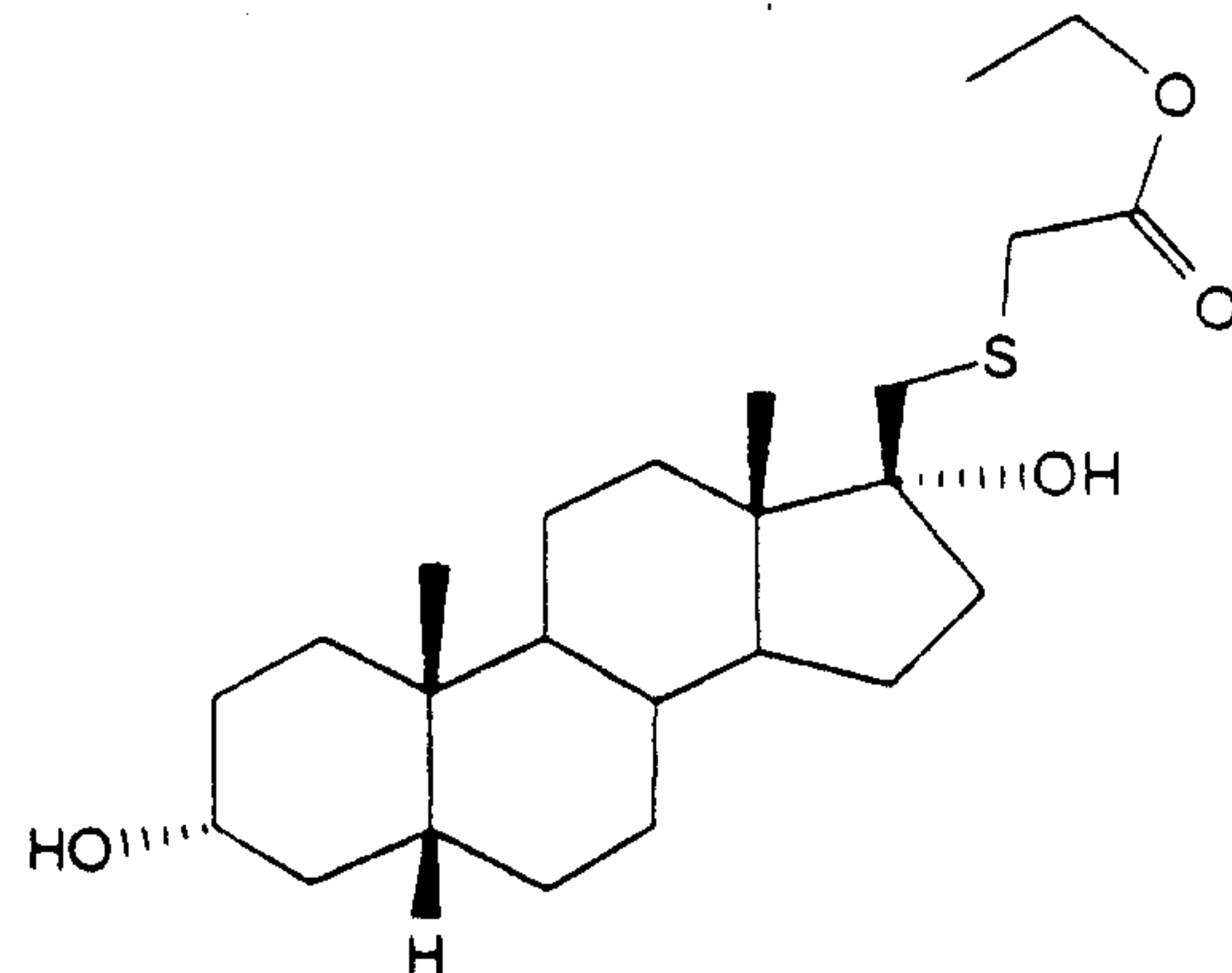
20-(CARBETHOXYMETHYL)THIO-21-NOR-5 \beta - PREGNAN-3 \alpha ,17 \alpha -DIOL
