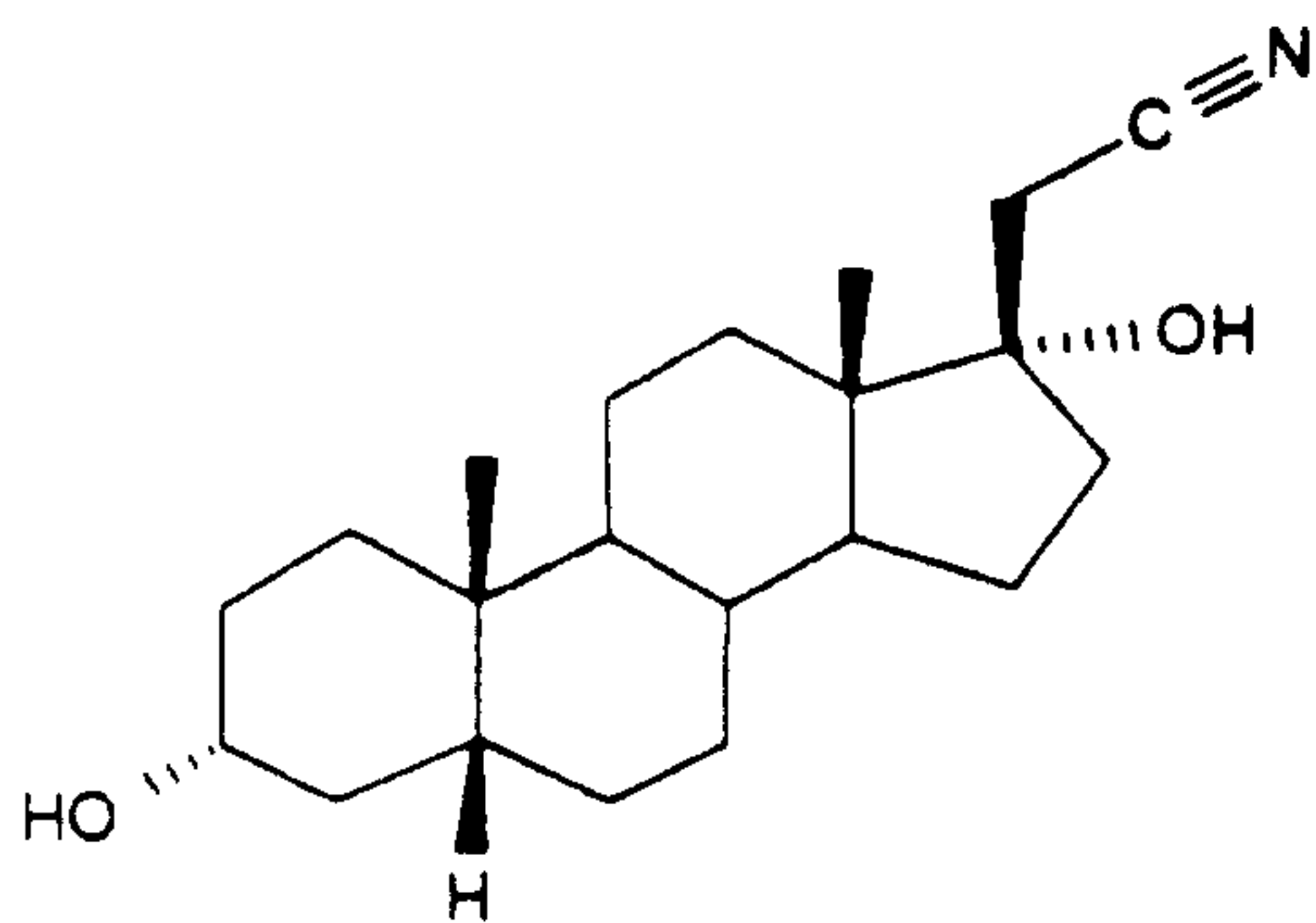
5 20-CYANO-21-NOR-5 \beta -PREGNAN-3 \alpha ,17 \alpha - DIOL
