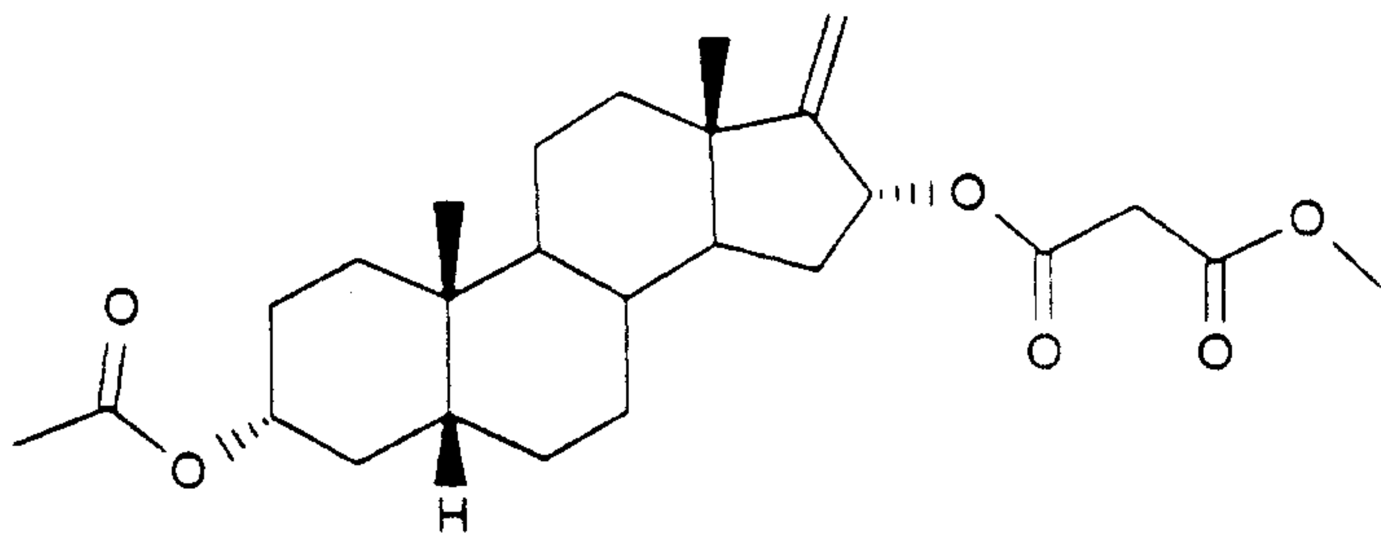
21-NOR-5 \beta -PREGN-17(20)-EN-3 \alpha , 16-DIOL-3-ACETATE-16-(O-METHYL)MALONATE
