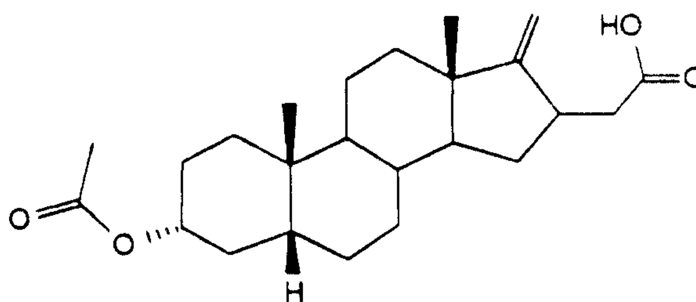
21-NOR-5 \beta -PREGN-17(20)-EN-3 \alpha -OL- 16-ACETIC ACID-3-ACETATE
