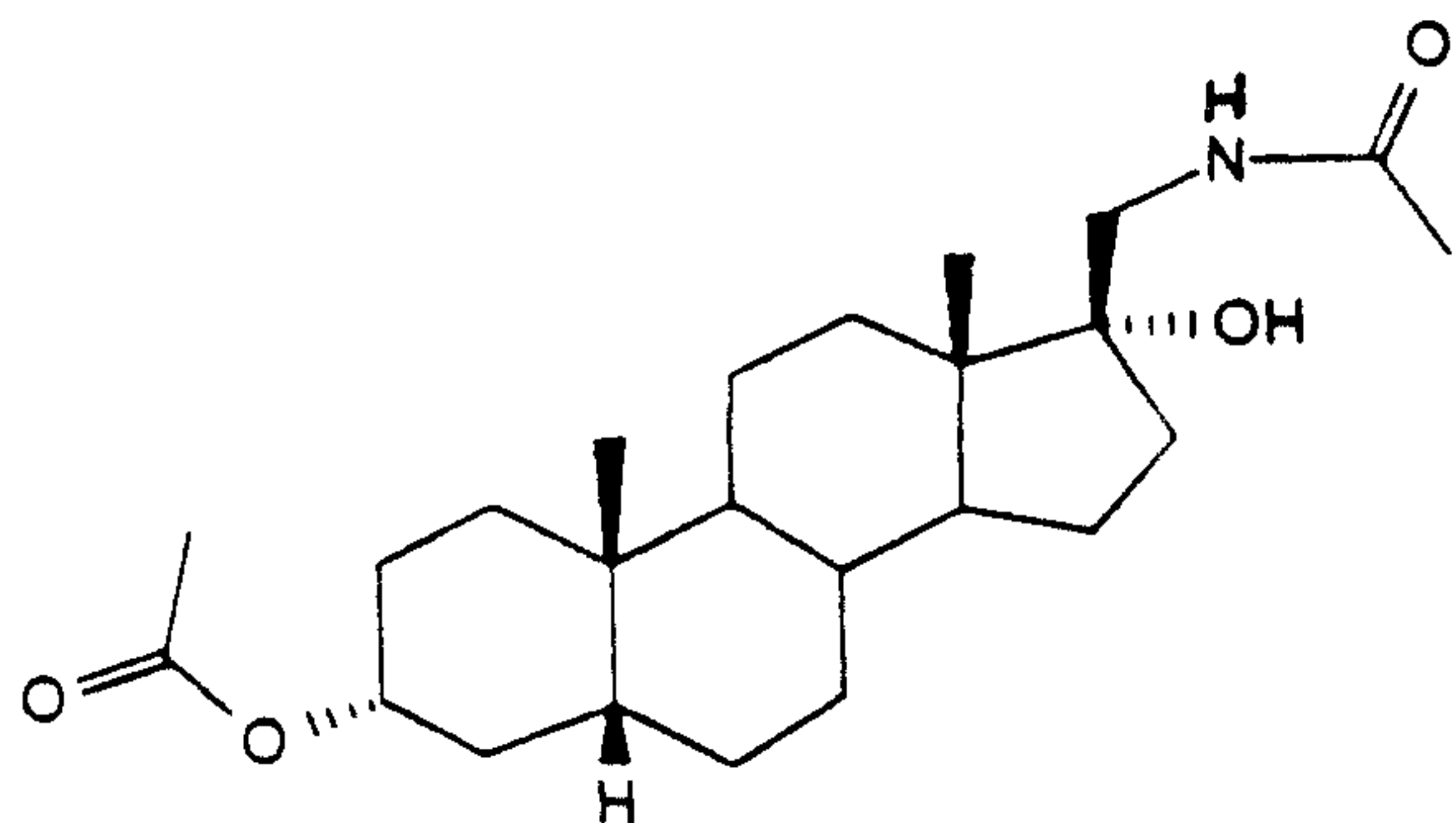
20-ACETAMIDO-21-NOR-5 \beta -PREGNAN-3 \alpha , 17 \alpha -DIOL-3-ACETATE
