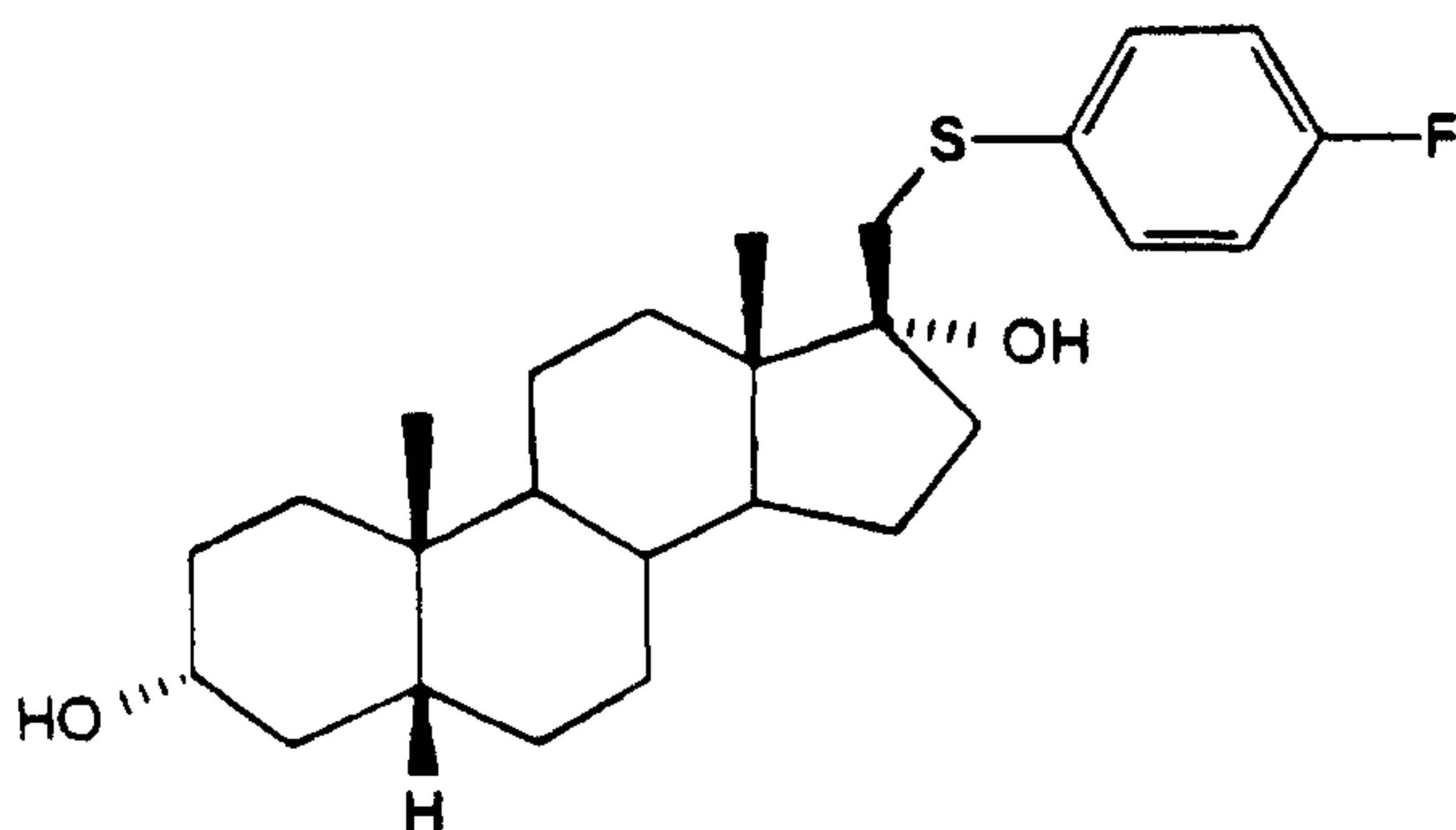
20-(4-FLUOROPHENYL)THIO-21-NOR- 5 \beta -PREGNAN-3 \alpha ,17 \alpha -DIOL
