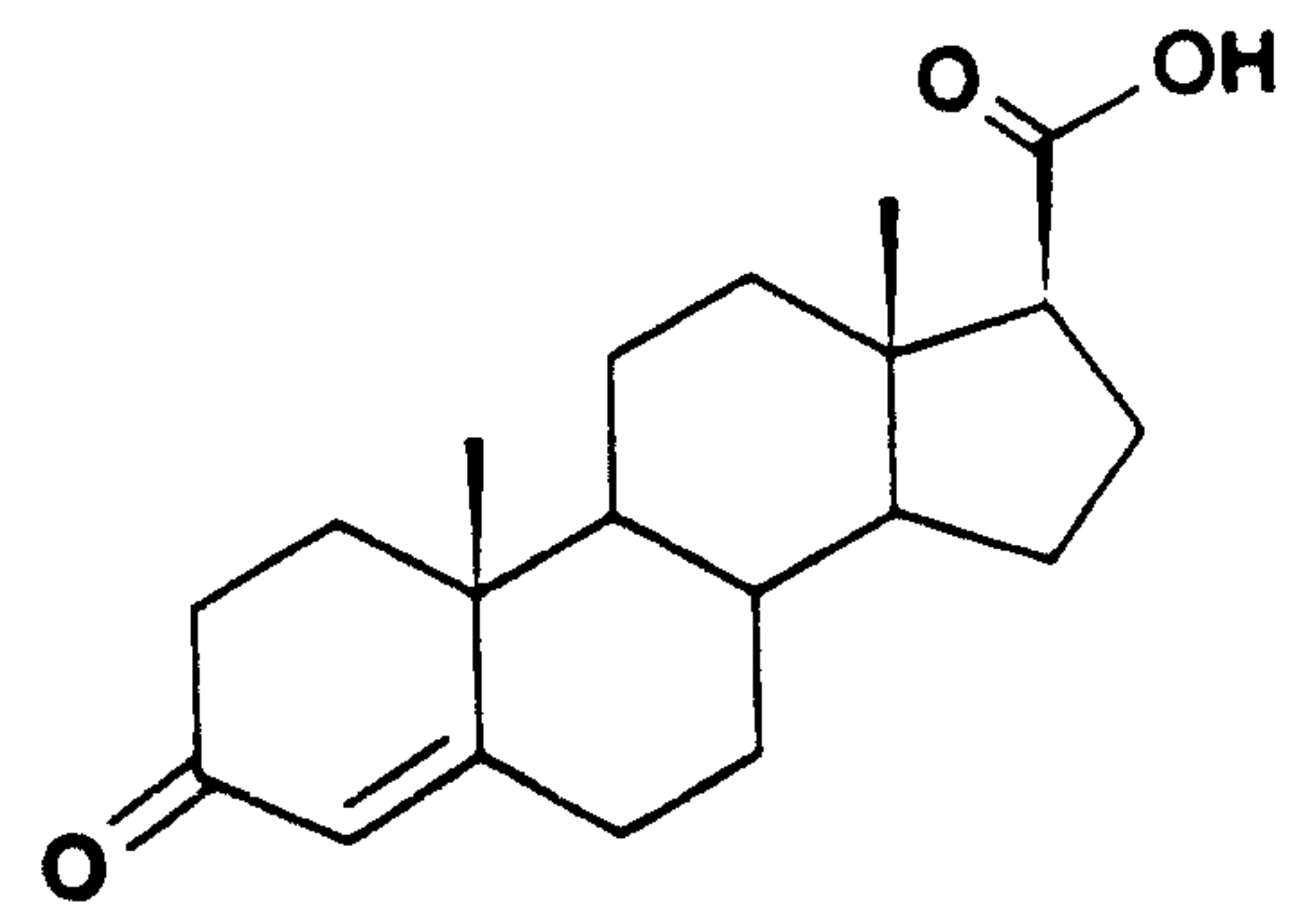
4-ANDROSTEN-3-ONE-17 \beta -CARBOXYLIC ACID
