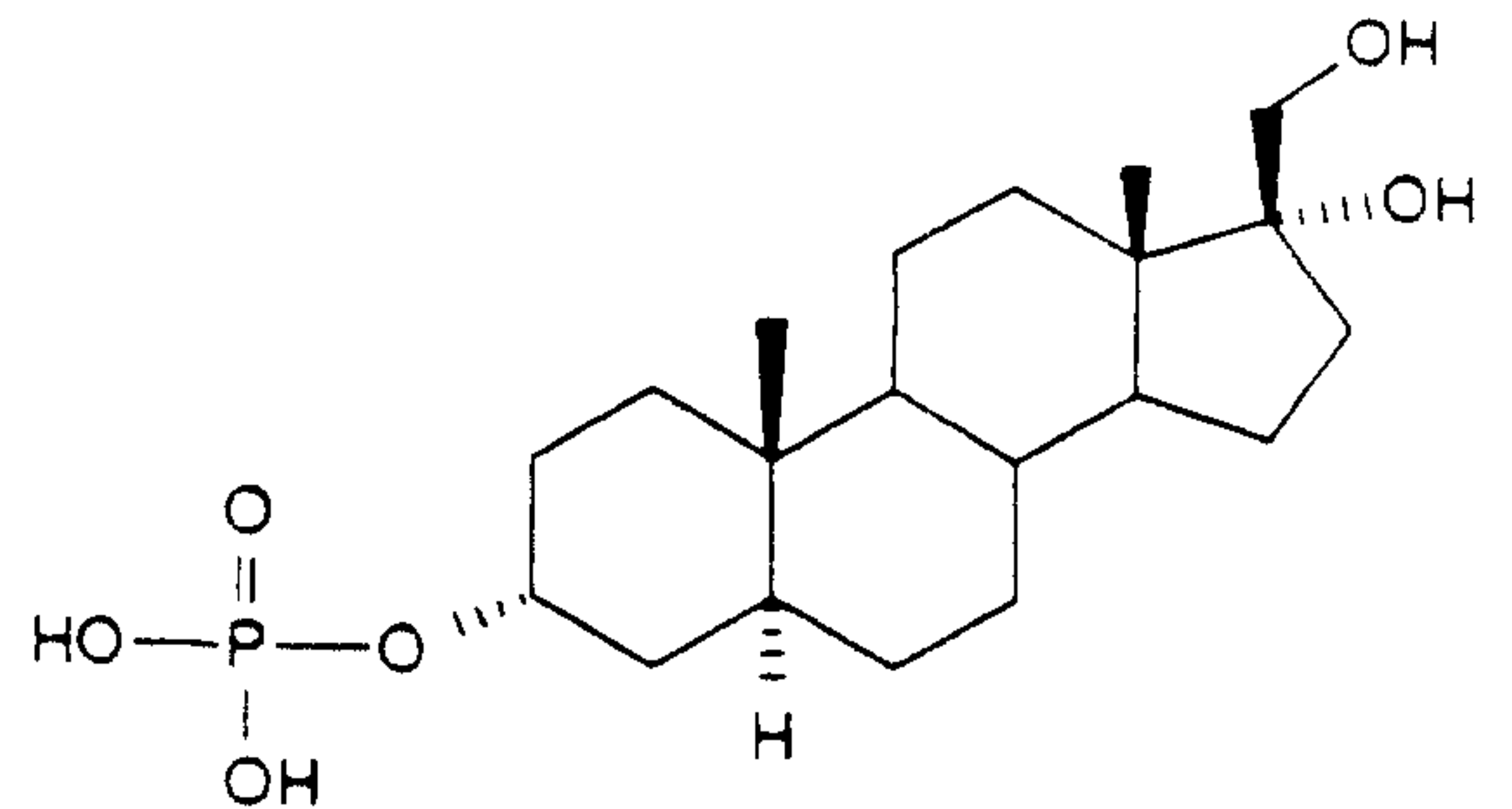
21-NOR-5 \alpha -PREGNAN-3 \alpha ,17 \alpha ,20-TRIOL- 3-PHOSPHATE
