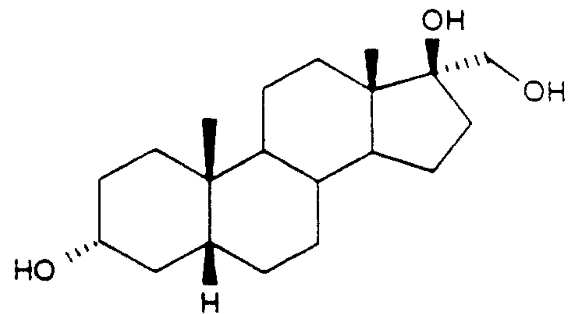
21-NOR-5 \beta -PREGNAN-3 \alpha ,17 \beta ,20-TRIOL
