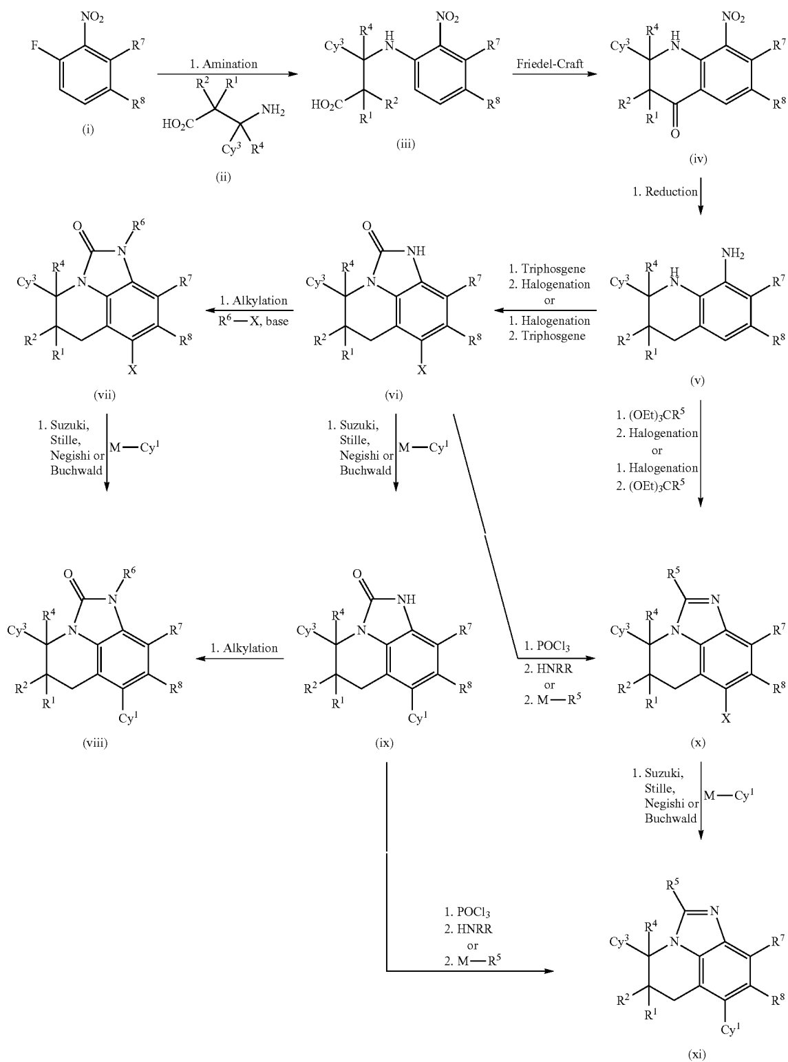
Scheme III
