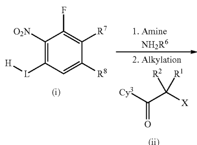
Scheme II
