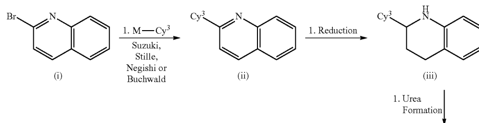
Scheme VIII
