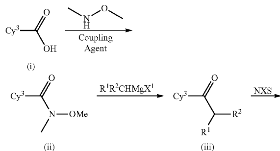
Scheme VII
