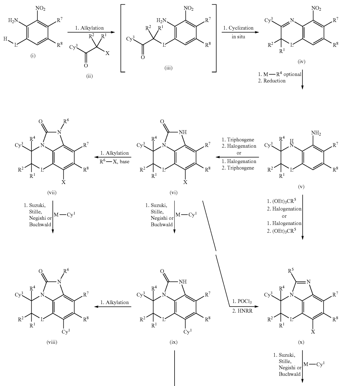
Scheme I
