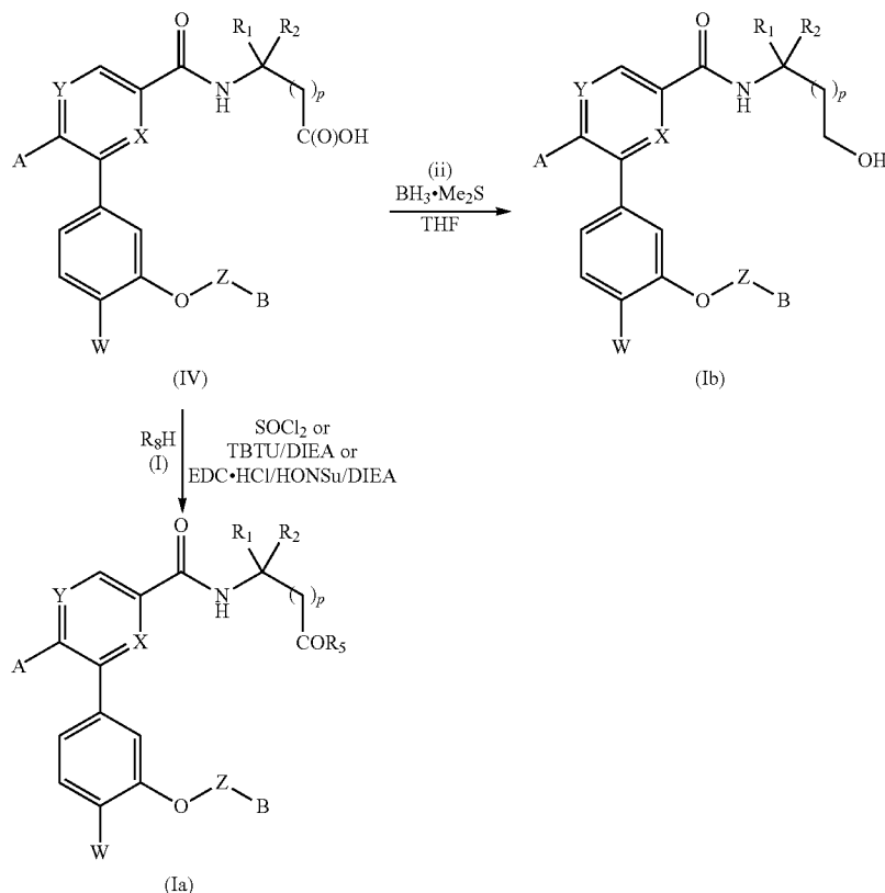
Synthetic scheme 2:
