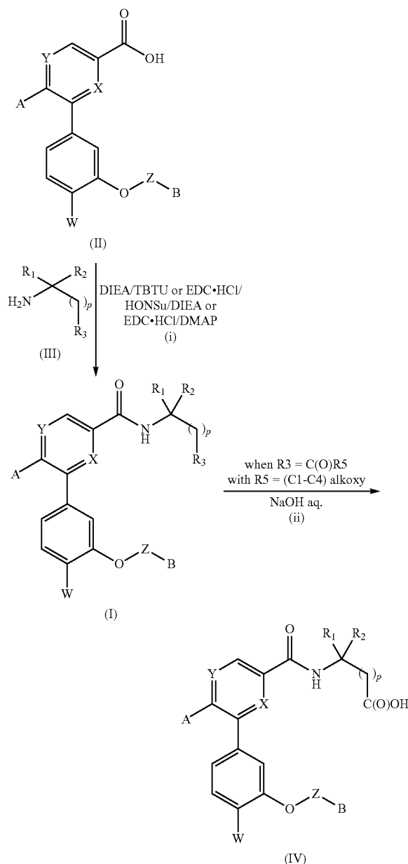
Synthetic scheme 1:
