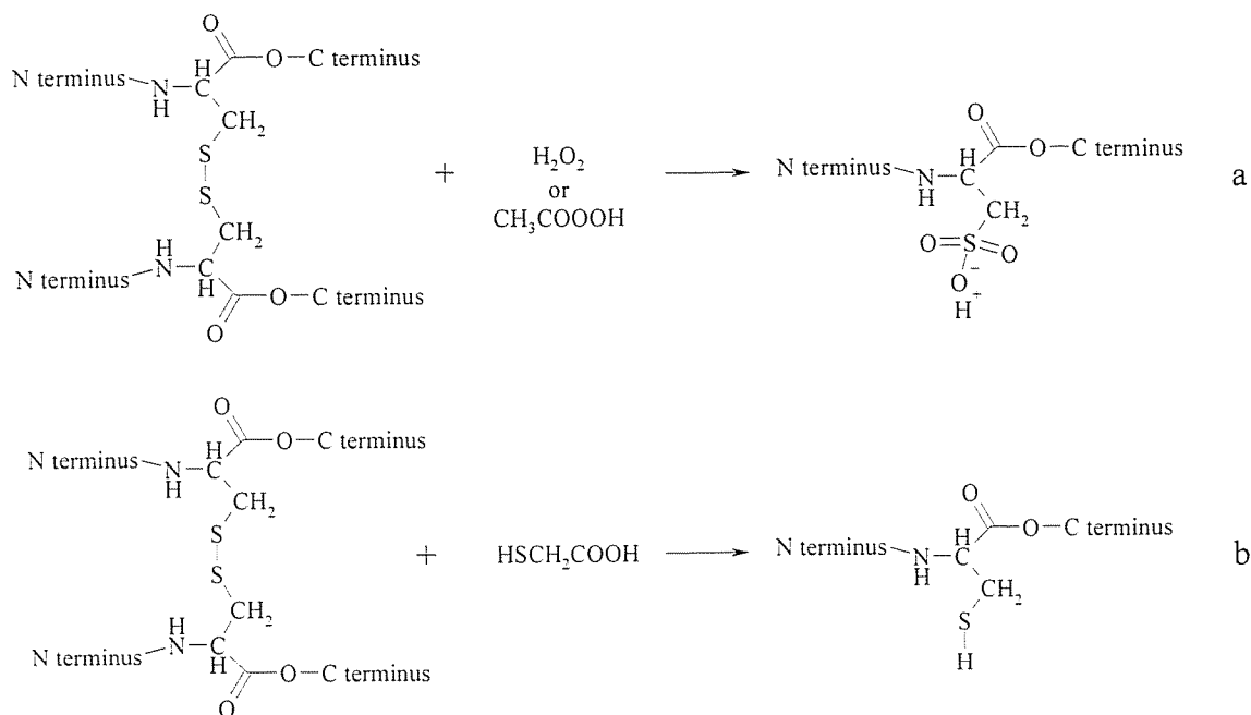
Scheme 1. General representations of (a) oxidation and (b) reduction of disulfide crosslinks in keratin. These reactions cleave the sulfur-sulfur bond in cystine residues, thereby destroying the superstructure and rendering the keratins soluble in the reaction media. The resultant fractions are keratose (a) and kerateine (b).
