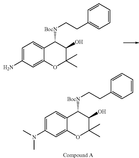
Compound A
