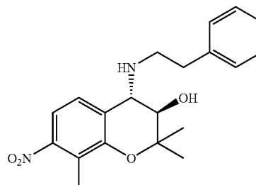
(3R*,4S*)-2,2,8-trimethyl-7-nitro-4-[(2-phenylethyl)amino]-3,4-dihydro-2H-1-benzopyran-3-ol
