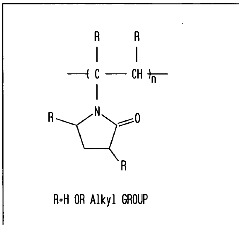
FIG. 1 MOLECULAR STRUCTURE OF GANEX V220 (PVP-EICOSANE COPOLYMER)
