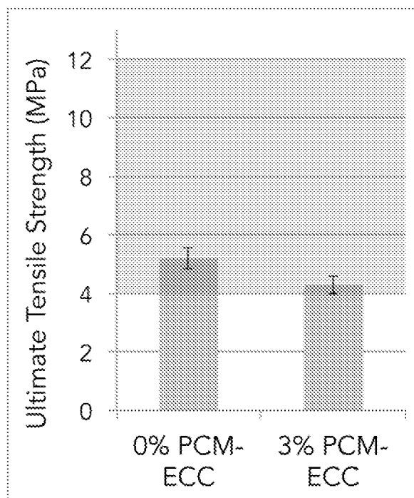
Figure 5. Ultimate tensile strength of 0% and 3% PCM-ECC mixes. Shaded grey area represents range previously attained with various ECC designs with corresponding compressive strength 20-90 MPa. Average and 95% confidence intervals shown.
