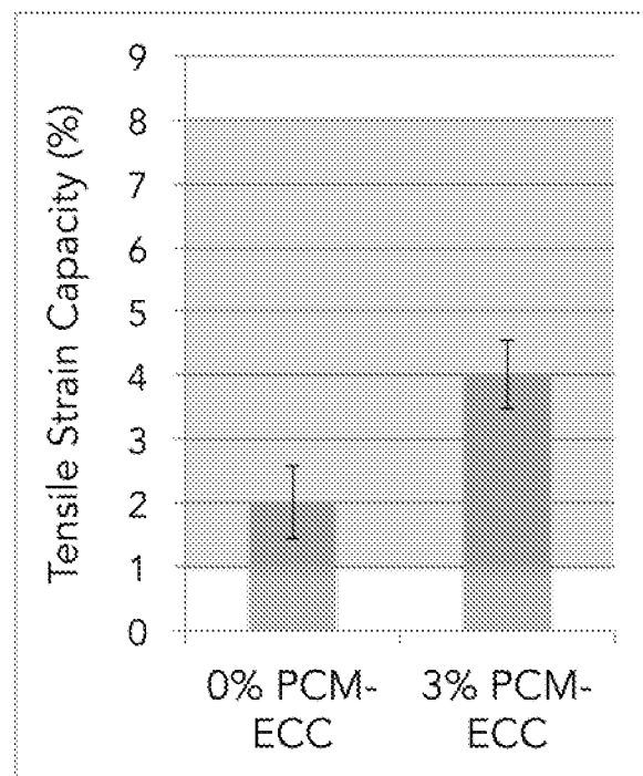
Figure 4. Tensile strain capacity of 0% and 3% PCM-ECC mixes. Shaded grey area represents range previously attained with various ECC designs with corresponding compressive strength 20-90 MPa. Average and 95% confidence intervals shown.
