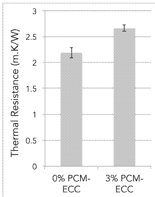
Figure 12. Specific thermal resistance of 0% and 3% PCM-ECC. Average and 95% confidence intervals shown.
