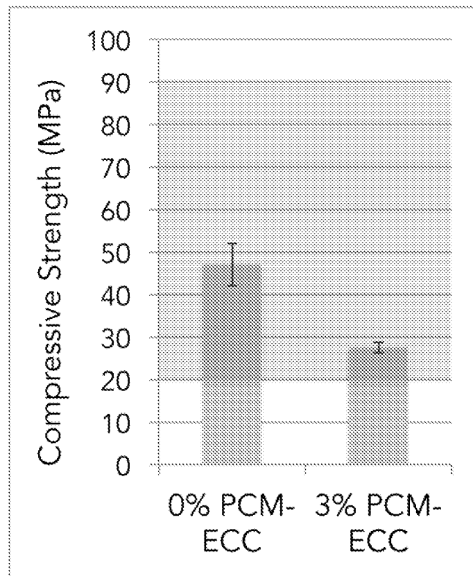
Figure 2. Compressive strength comparison between 0% and 3% PCM-ECC averages. The 95% confidence intervals are indicated as error bars. Shaded region demarcates attainable range with ECC referenced in Li, M. and Li, V.C. in "Rheology, fiber dispersion, and robust properties of Engineered Cementitious Composites," Materials and Structures, DOI:10.1617/s11527-012-9909-z, 2012.
