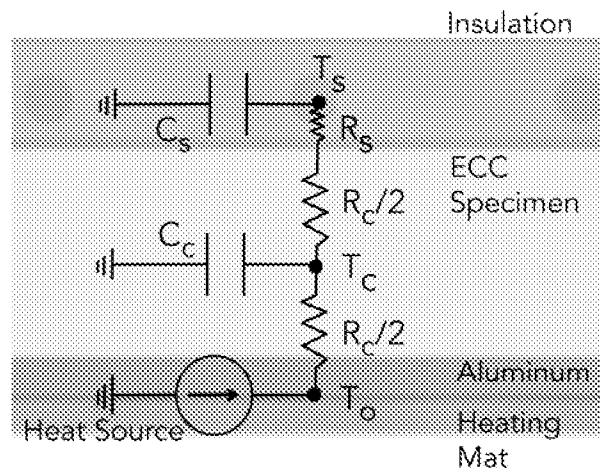
Figure 11. Thermal equivalent circuit used to model heat transfer through the assembly.
