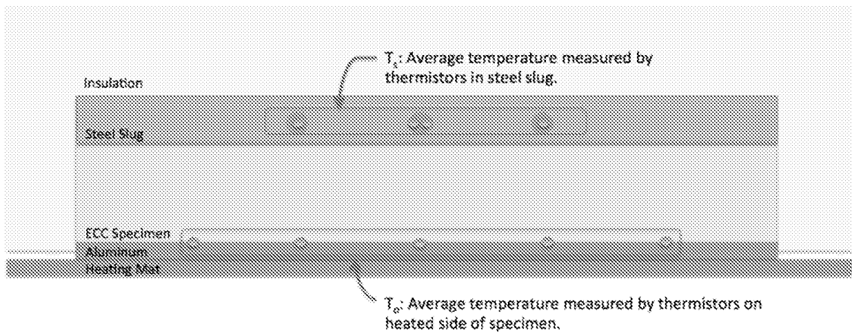
Figure 10. Diagram of thermal resistance test setup and thermistor locations.
