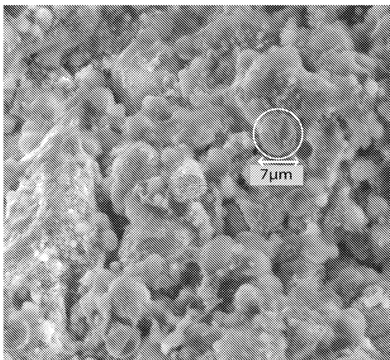
Figure 1. SEM image of a 3% PCM-ECC specimen. Diameter and location of one PCM capsule indicated above.
