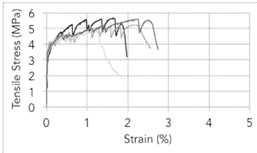
Figure 6. Stress-strain diagram of 0% PCM-ECC under uniaxial tension.
