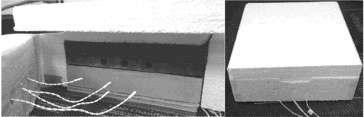
Figure 9. Image of interior of thermal resistance test setup (left), and closed apparatus (right).
