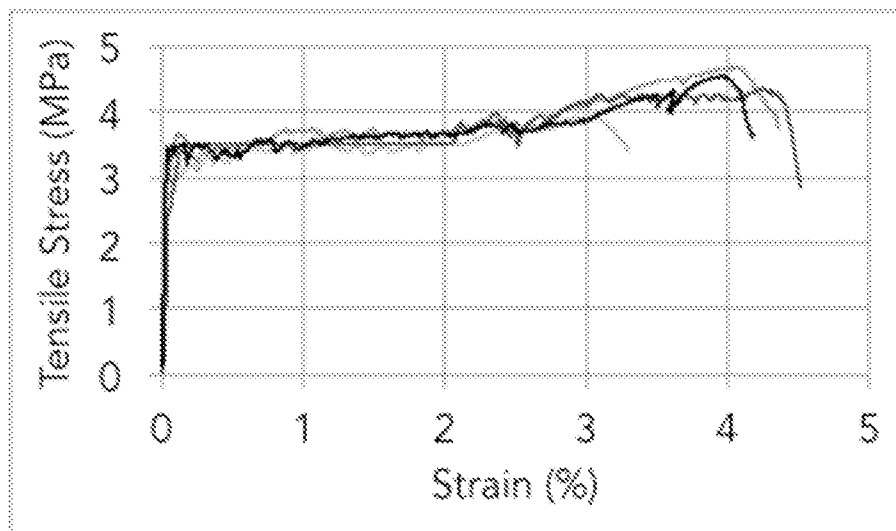
Figure 7. Stress-strain diagram of 3% PCM-ECC under uniaxial tension. The linear elastic behavior gives way to significant strain hardening post first-cracking due to PCM addition.
