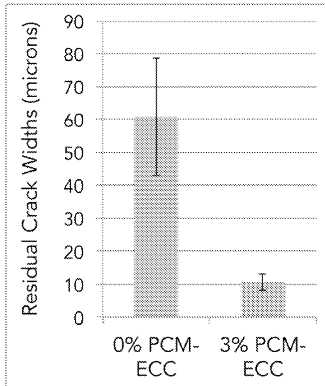
Figure 3. Residual crack widths of 0% and 3% PCM-ECC specimens after uniaxial tension tests were conducted. Average and 95% confidence intervals shown.
