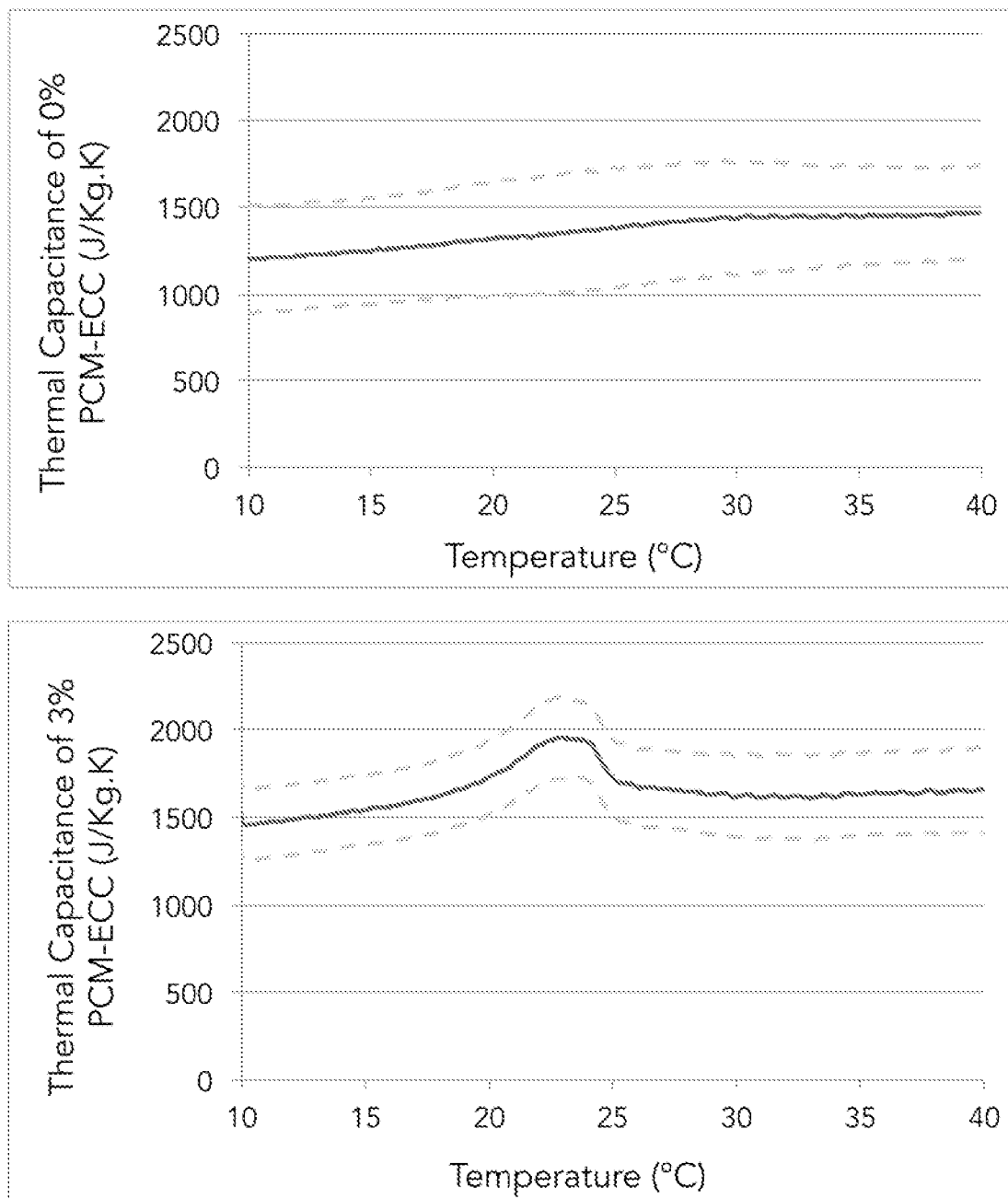
Figure 8. Specific heat capacity profiles of 0% and 3% PCM-ECC as determined by DSC. Solid lines depict 4-specimen average; dashed lines depict 95% confidence intervals.
