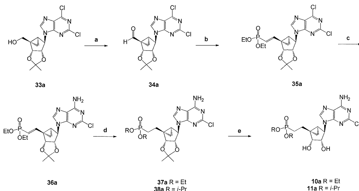
Scheme 4a
