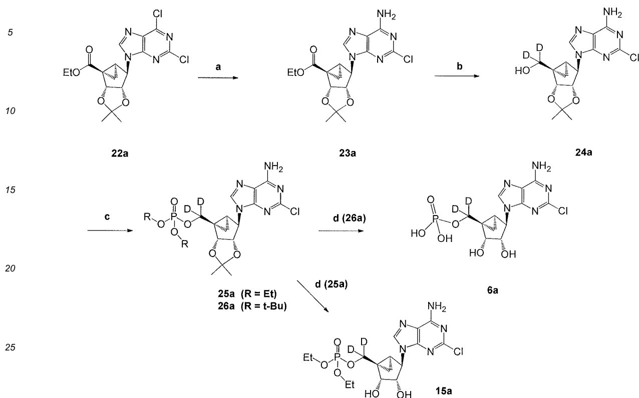
Scheme 3a
