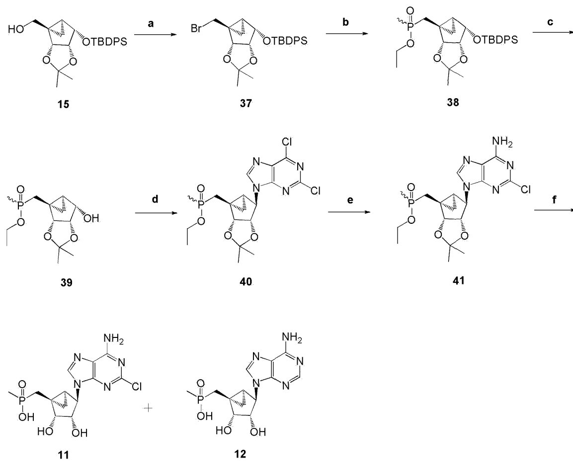
Scheme 6
