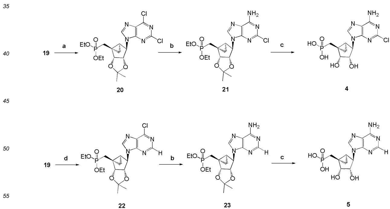
Scheme 2
