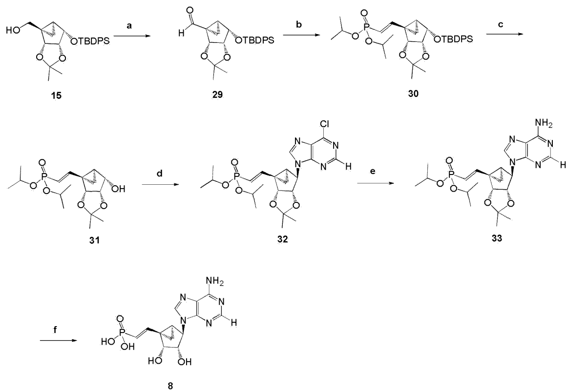
Scheme 5
