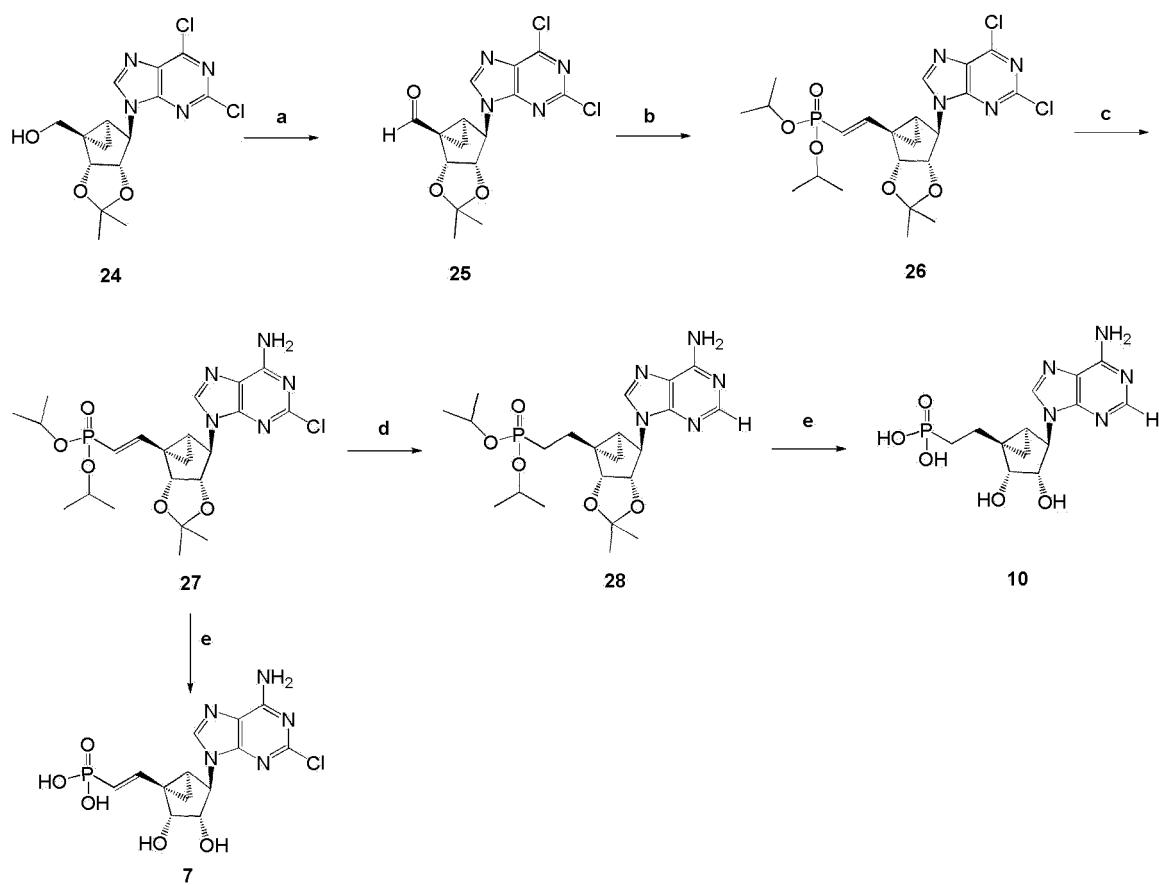
Scheme 3
