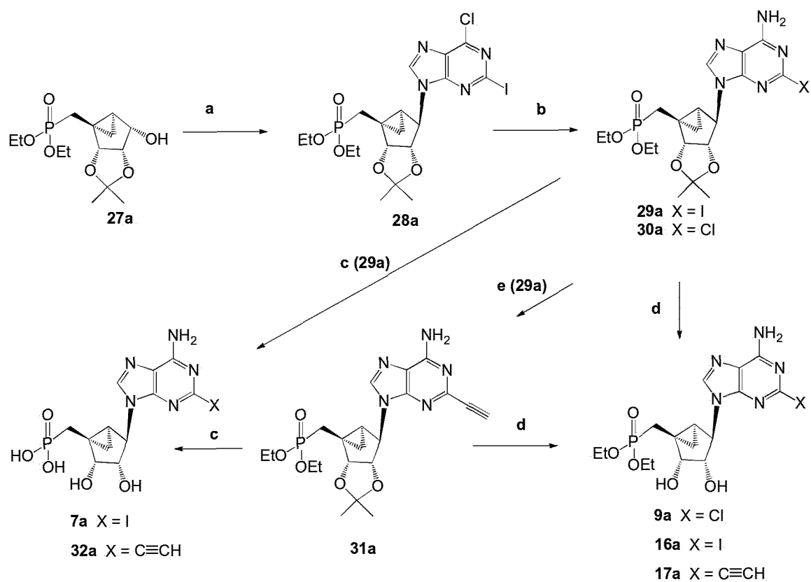
Scheme 4a
