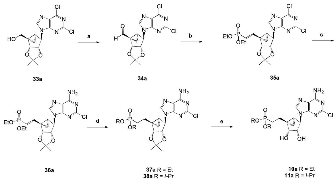
Scheme 4a
