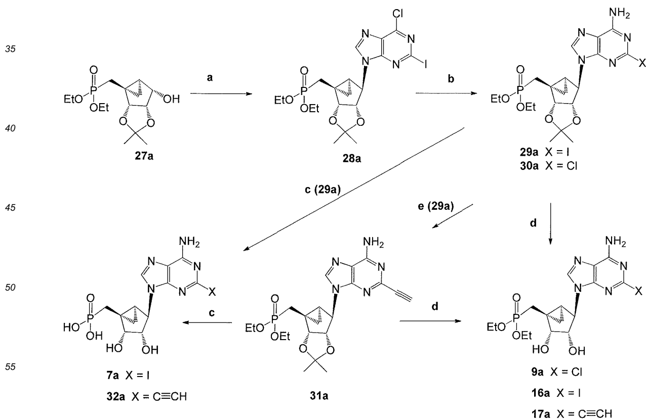
Scheme 3a
