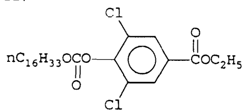
(Cpd - 12)
