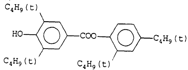
(Cpd - 3)
