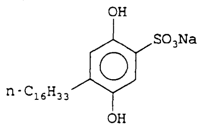
(Cpd - 13)
