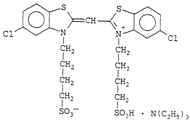
(ExS - 6)
