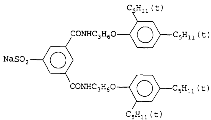
(Cpd - E)
