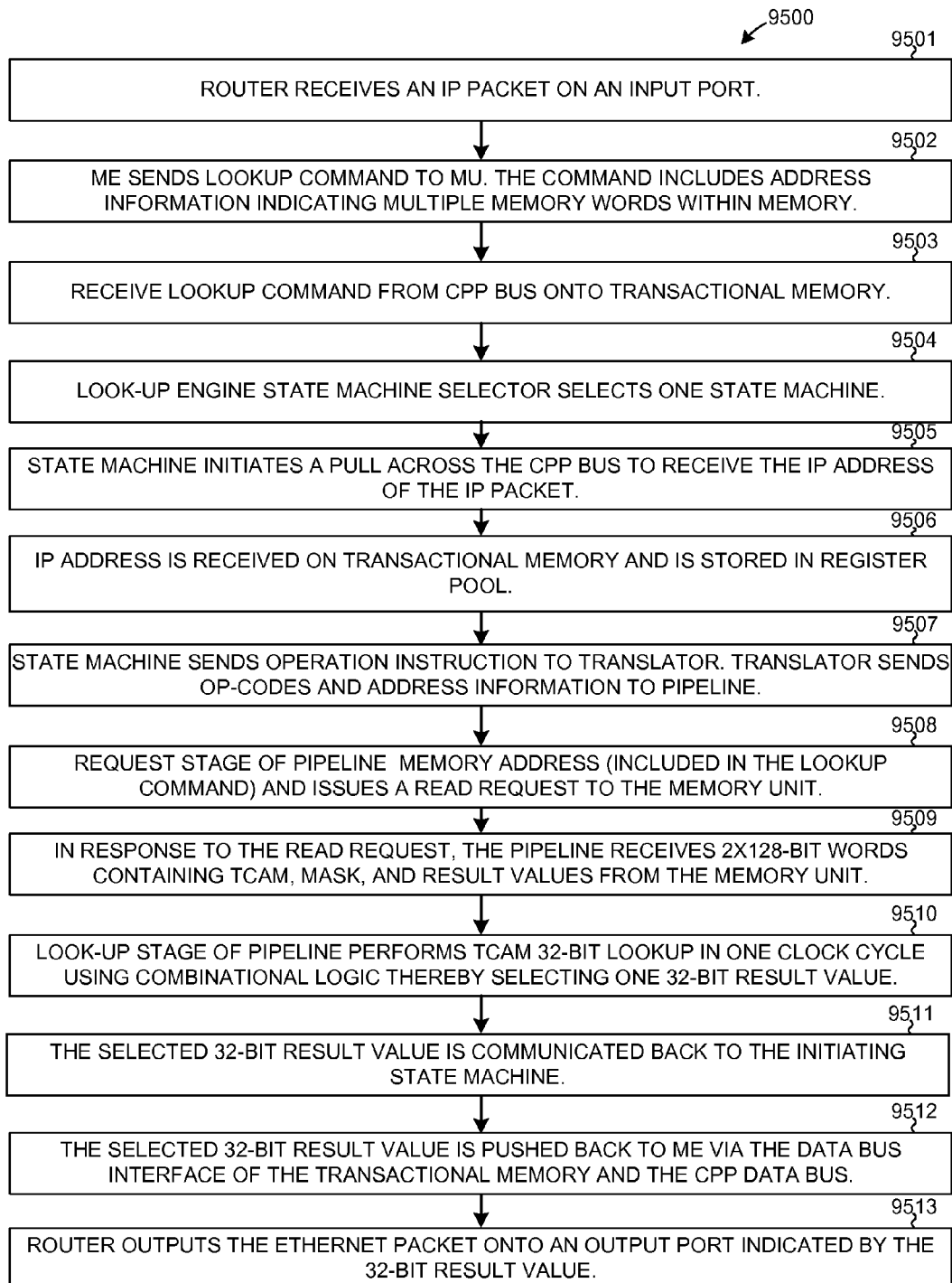
TCAM 32 BIT LOOK-UP FLOWCHART FIG. 55
