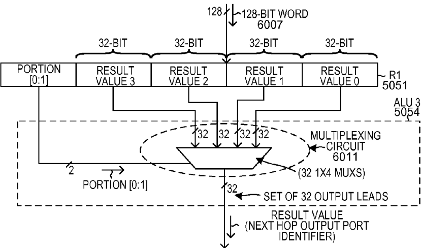
DIRECT 32-BIT LOOKUP STAGE FIG. 42
