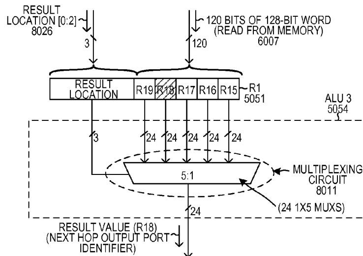
DIRECT 24-BIT LOOK-UP STAGE FIG. 49
