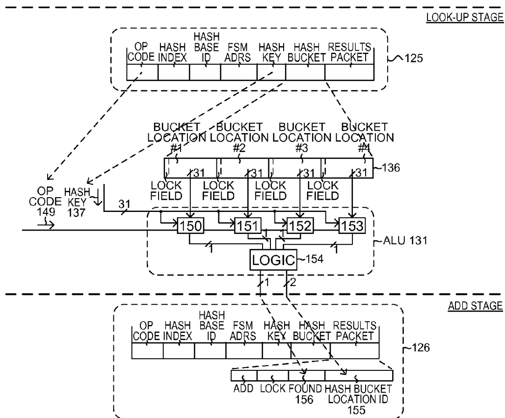
LOOK-UP STAGE FIG. 20
