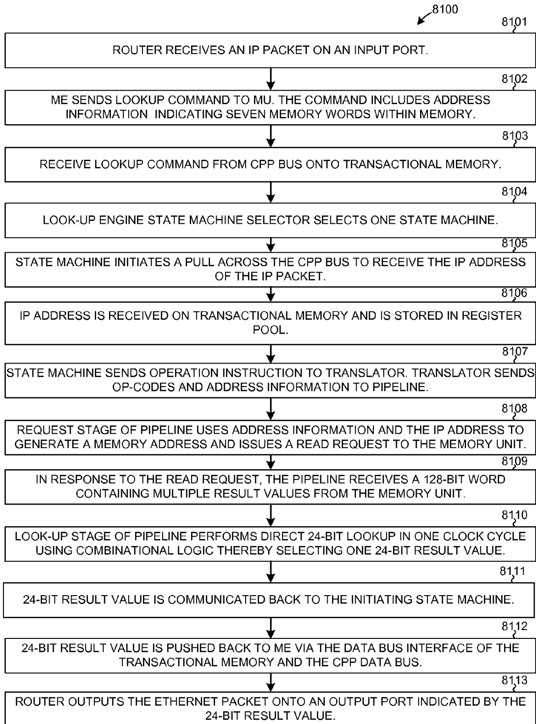
DIRECT 24-BIT LOOK-UP FLOWCHART
