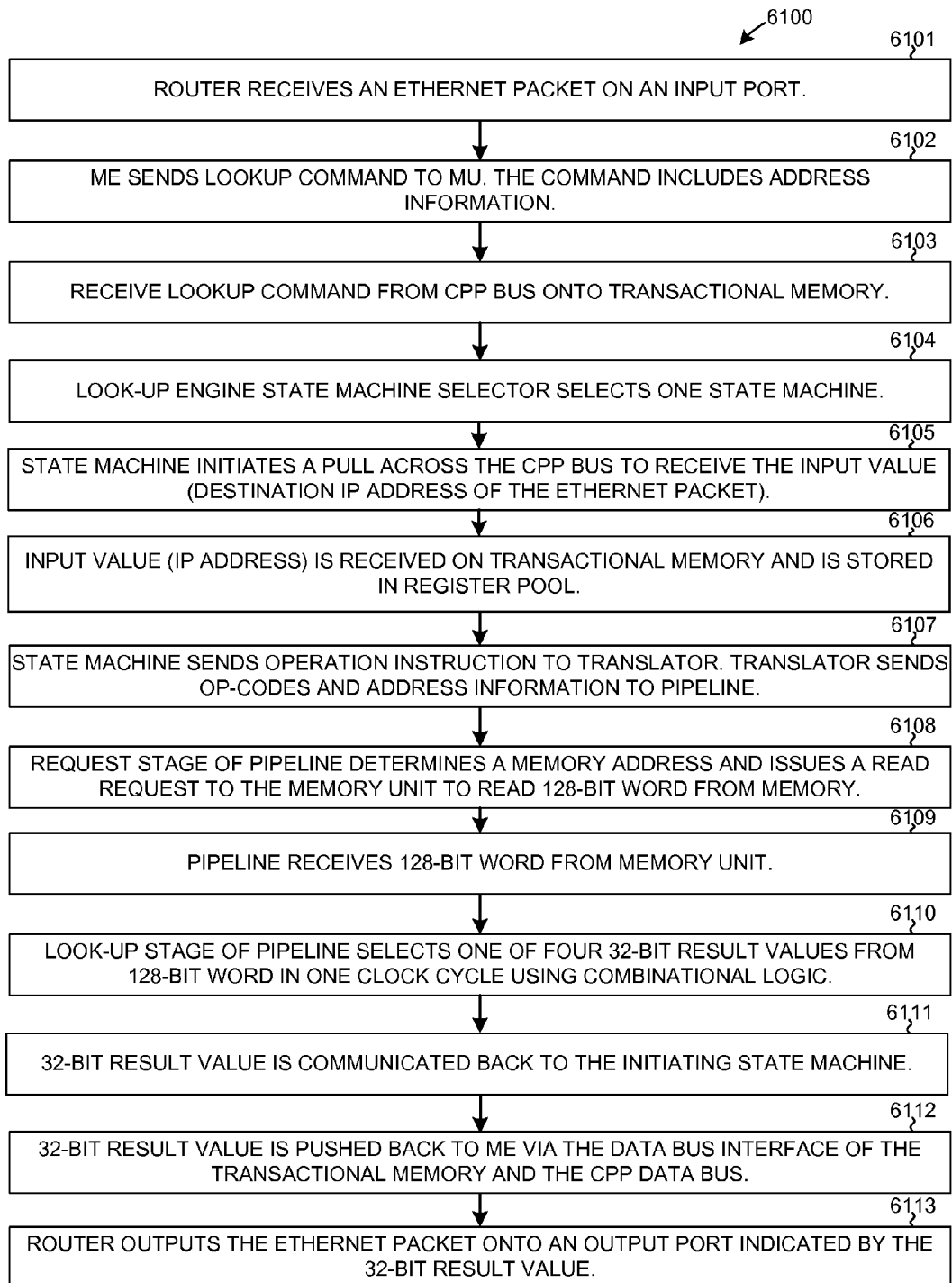
DIRECT 32-BIT LOOKUP FLOWCHART
