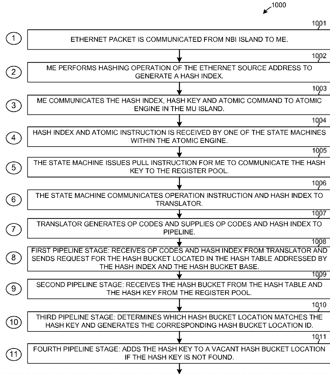
TRANSACTIONAL MEMORY FLOWCHART FIG. 22A
