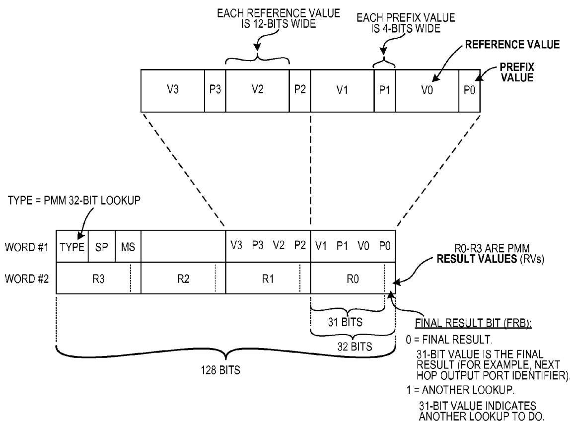
2X128 BITS READ OUT OF MEMORY UNIT FIG. 57
