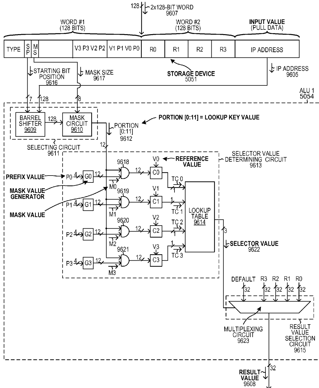
LOOKUP STAGE PERFORMING PMM 32-BIT LOOKUP FIG. 59
