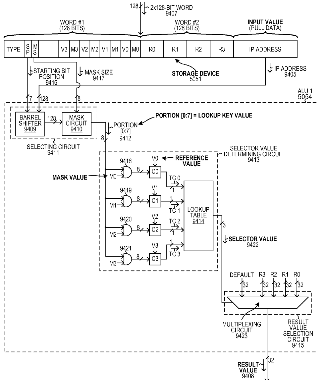
LOOKUP STAGE PERFORMING TCAM 32-BIT LOOKUP FIG. 53
