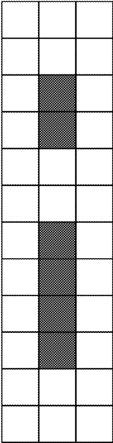
Intended Data
