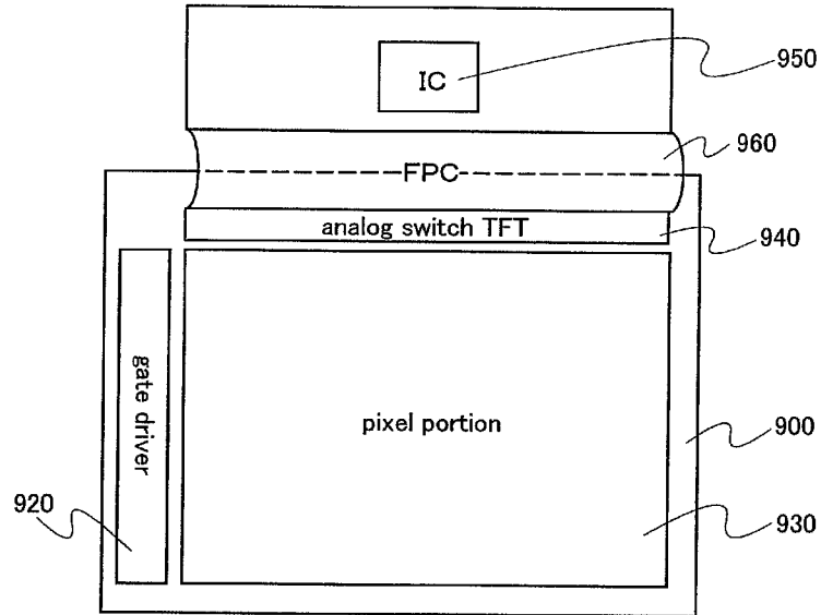
FIG. 17A IC connected by FPC
