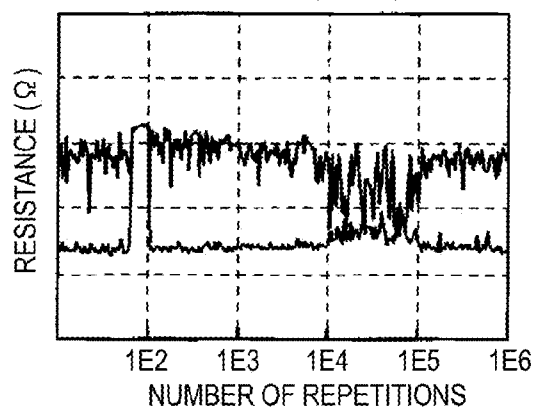
SMALL T_r ( 50 \mu A )
