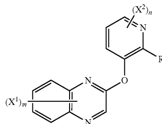
[Chemical Formula 17]
