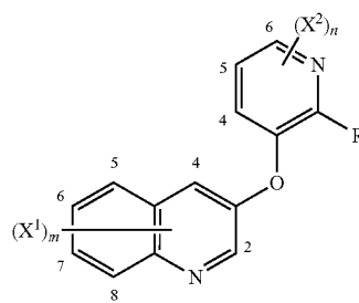
[Chemical Formula 50]
