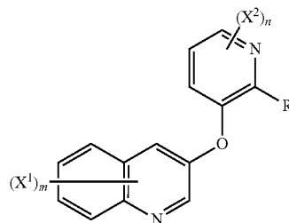
[Chemical Formula 15]
