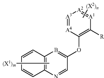
[Chemical Formula 13]
