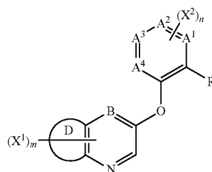
[Chemical Formula 6]
