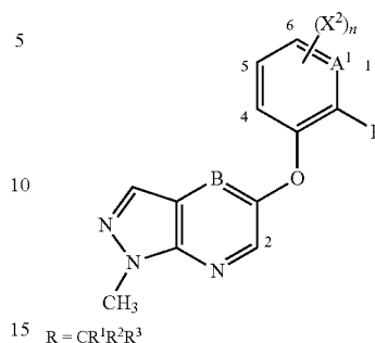
[Chemical Formula 55]
