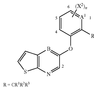
[Chemical Formula 54]
