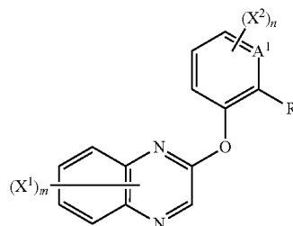
[Chemical Formula 16]
