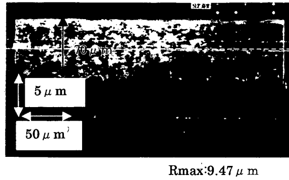
Fig.10(B) (After CZ roughing processing)
