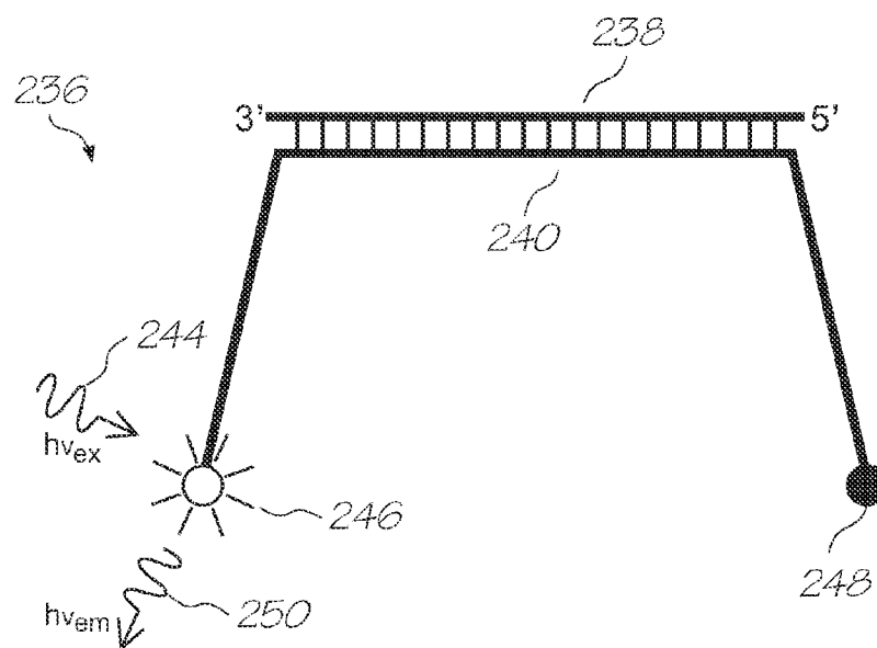
FIG. 59 (PRIOR ART)
