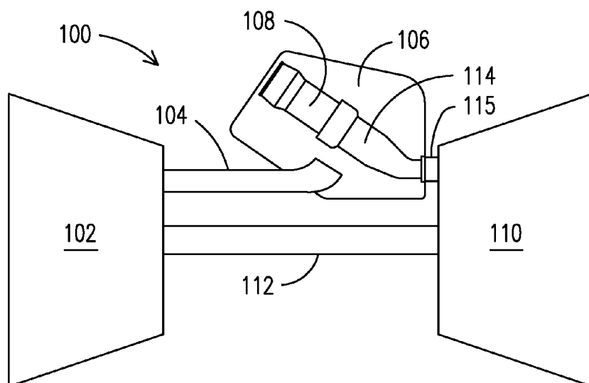
FIG. 1 PRIOR ART
