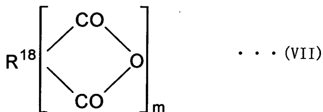
[Chemical Formula 3]
