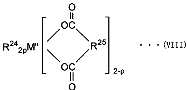
[Chemical Formula 4]
