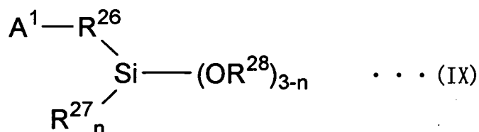
[Chemical Formula 5]
