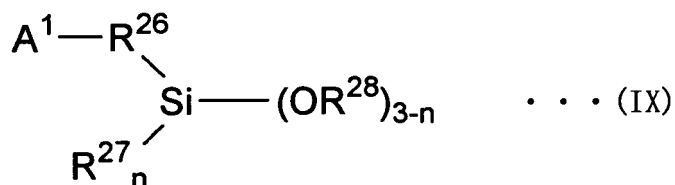
[Chemical Formula 5]
