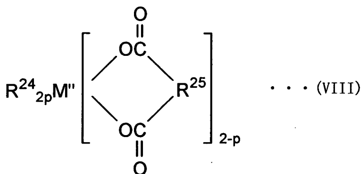
[Chemical Formula 4]
