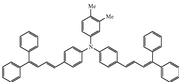
Compound ( \gamma )
