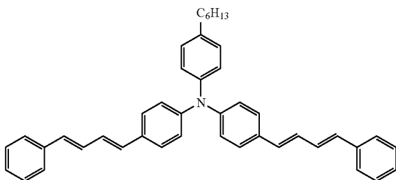
Compound ( \beta )
