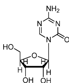
Azacitidine
