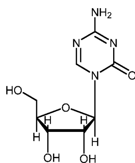
Azacitidine
