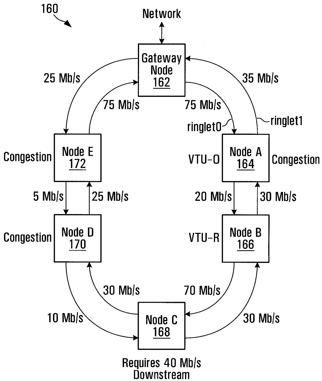
Migration of Ring Network Conditions Over Time
