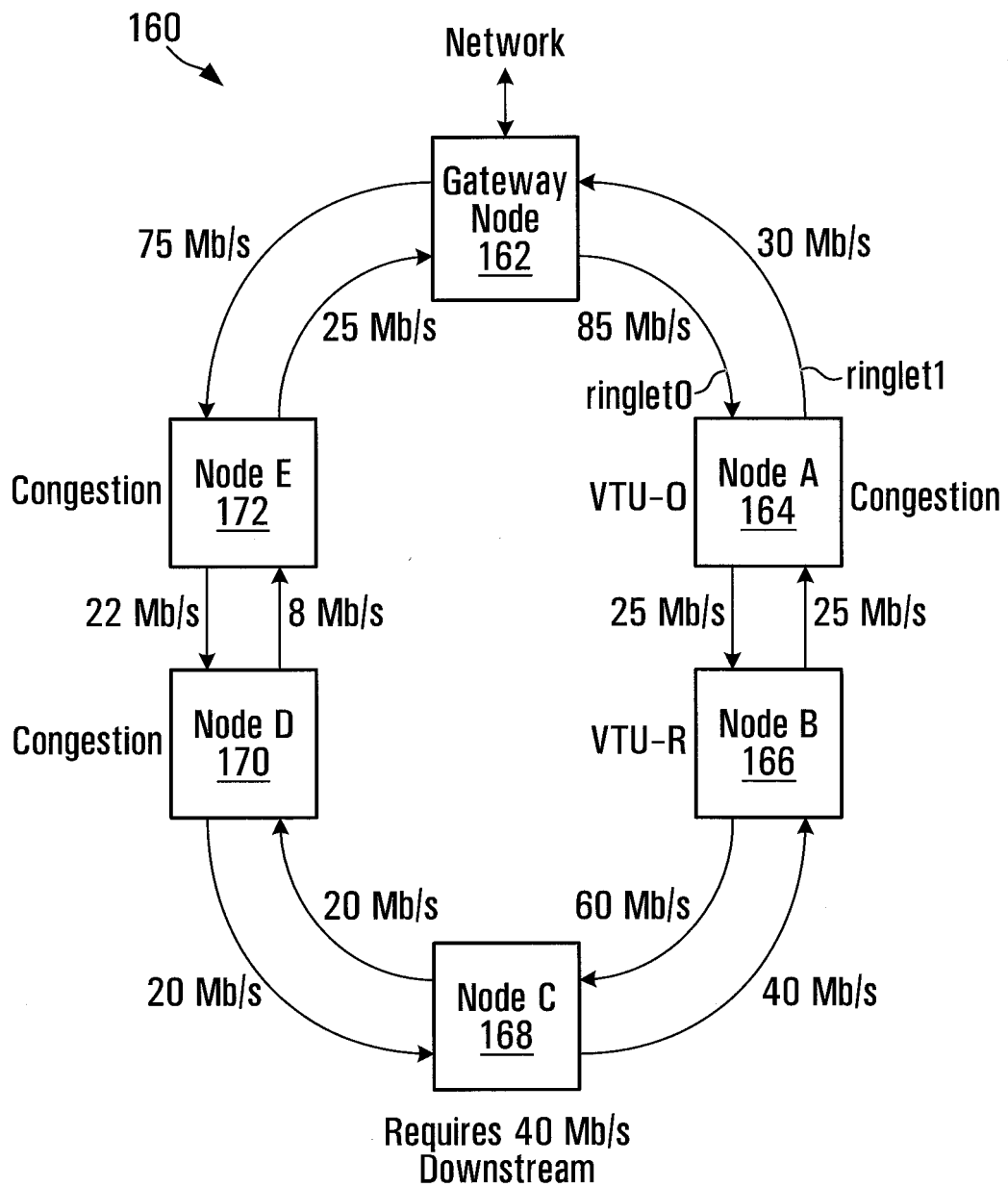
Asymmetric DSL Rings Dynamically Optimized Ring
