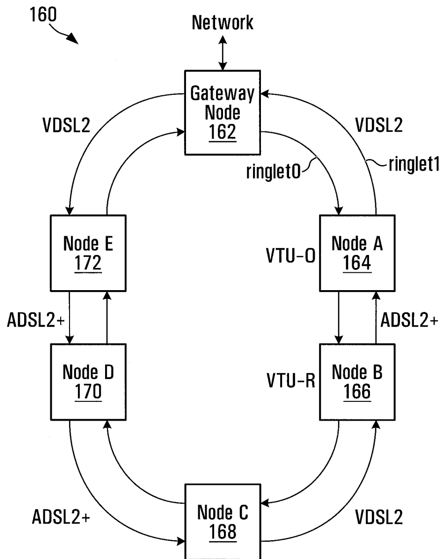
Deployment of Mixed xDSL Links in a DSL Ring Configuration
