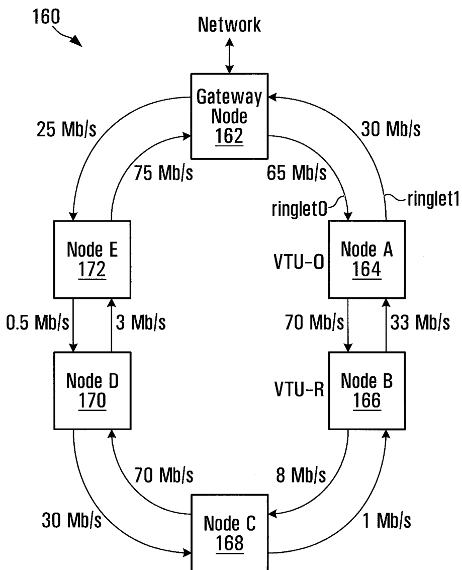
Ring with Inherent Bandwidth Bottlenecks
