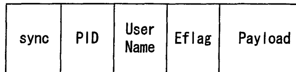
FIG. 17 (A) PARENT DEVICE PACKET (BRAODCASTING DATA)
