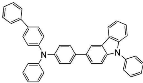
PCBA1BP
