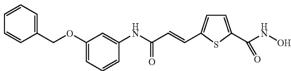
5-[2-(3-Benzyloxy-phenylcarbamoyl)-vinyl]-thiophene-2-carboxylic acid hydroxyamide
