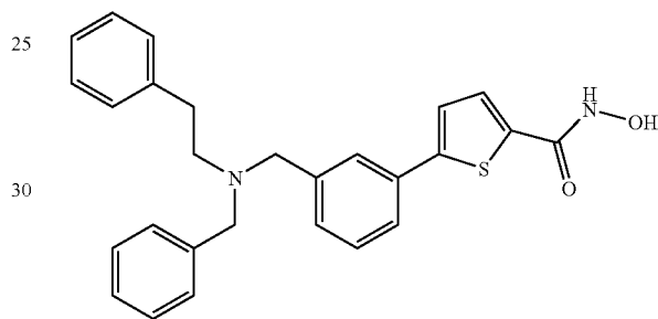
5-{3-[(Benzyl-phenethyl-amino)-methyl]-phenyl}-thiophene-2-carboxylic acid hydroxyamide
