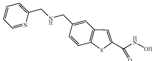
5-[(Pyridin-2-ylmethyl)-amino]-methyl}-benzo[b]thiophene-2-carboxylic acid hydroxyamide
