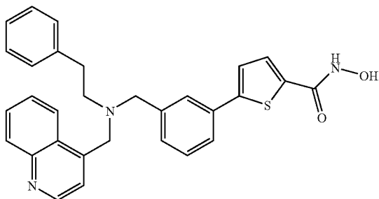
5-{3-[(Phenethyl-quinolin-4-ylmethyl-amino)-methyl]-phenyl}-thiophene-2-carboxylic acid hydroxyamide
