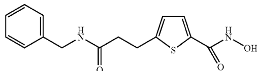
5-(2-Benzylcarbamoyl-ethyl)-thiophene-2-carboxylic acid hydroxyamide
