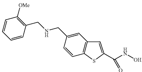
5-[(2-Methoxy-benzylamino)-methyl]-benzo[b]thiophene-2-carboxylic acid hydroxyamide
