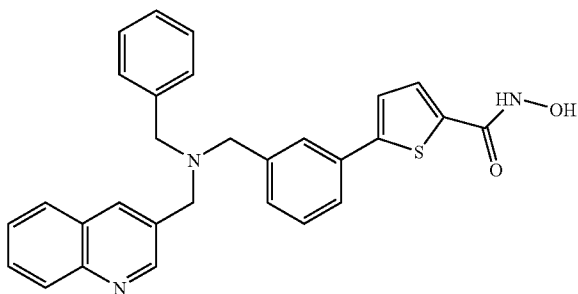
5-{3-[(Benzyl-quinolin-3-ylmethyl-amino)-methyl]-phenyl}-thiophene-2-carboxylic acid hydroxyamide
