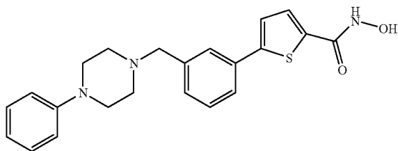
5-{3-[(4-Phenyl-piperazin-1-ylmethyl)-phenyl]-thiophene-2-carboxylic acid hydroxyamide
