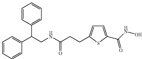
5-[2-(2,2-Diphenyl-ethylcarbamoyl)-ethyl]-thiophene-2-carboxylic acid hydroxyamide
