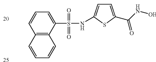
5-(Naphthalene-1-sulfonylamino)-thiophene-2-carboxylic acid hydroxyamide
