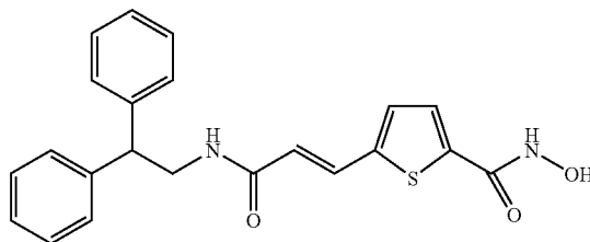
5-[2-(2,2-Diphenyl-ethylcarbamoyl)-vinyl]-thiophene-2-carboxylic acid hydroxyamide
