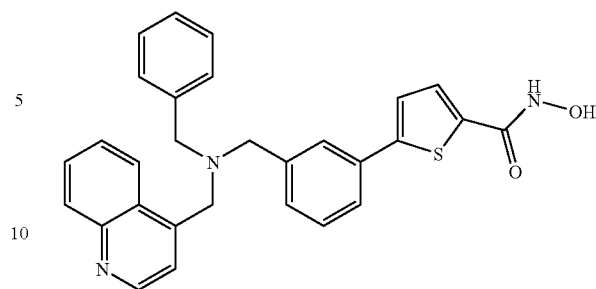
5-{3-[(Benzyl-quinolin-4-ylmethyl-amino)-methyl]-phenyl}-thiophene-2-carboxylic acid hydroxyamide
