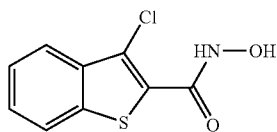
3-Chloro-benzo[b]thiophene-2-carboxylic acid hydroxyamide
