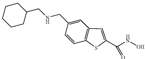
5-[(Cyclohexylmethyl-amino)-methyl]-benzo[b]thiophene-2-carboxylic acid hydroxyamide
