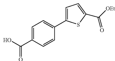
5-(4-Carboxy-phenyl)-thiophene-2-carboxylic acid ethyl ester
