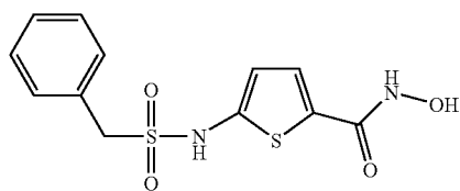
5-Phenylmethanesulfonylamino-thiophene-2-carboxylic acid hydroxyamide
