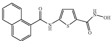
5-[(Naphthalene-1-carbonyl)-amino]-thiophene-2-carboxylic acid hydroxyamide
