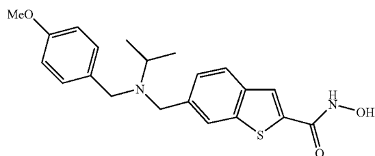
6-[[Isopropyl-(4-methoxy-benzyl)-amino]-methyl]- benzo[b]thiophene-2-carboxylic acid hydroxyamide
