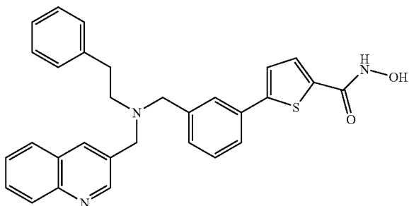
5-{3-[(Phenethyl-quinolin-3-ylmethyl-amino)-methyl]-phenyl}-thiophene-2-carboxylic acid hydroxyamide
