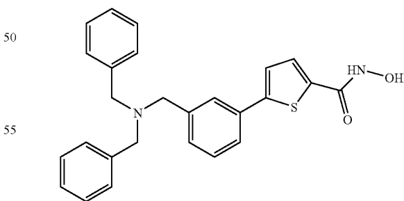
5-{3-[(Dibenzylamino)-methyl]-phenyl}-thiophene-2-carboxylic acid hydroxyamide
