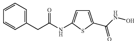
5-Phenylacetyl-amino-thiophene-2-carboxylic acid hydroxyamide
