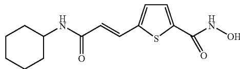
5-(2-Cyclohexylcarbamoyl-vinyl)-thiophene-2-carboxylic acid hydroxyamide
