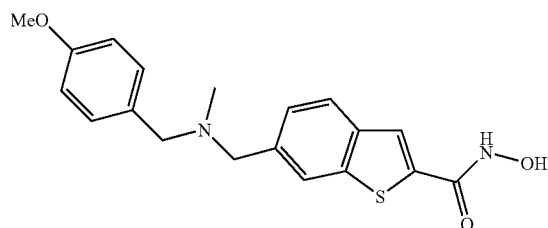
6-[[[4-Methoxy-benzyl)-methyl-amino]-methyl]- benzo[b]thiophene-2-carboxylic acid hydroxyamide
