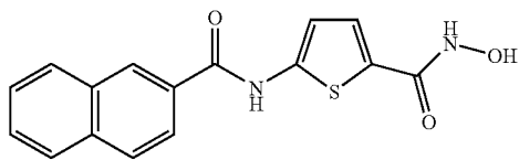
5-[(Naphthalene-2-carbonyl)-amino]-thiophene-2-carboxylic acid hydroxyamide
