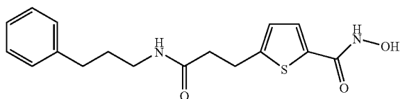
5-[2-(3-Phenyl-propylcarbamoyl)-ethyl]-thiophene-2-carboxylic acid hydroxyamide
