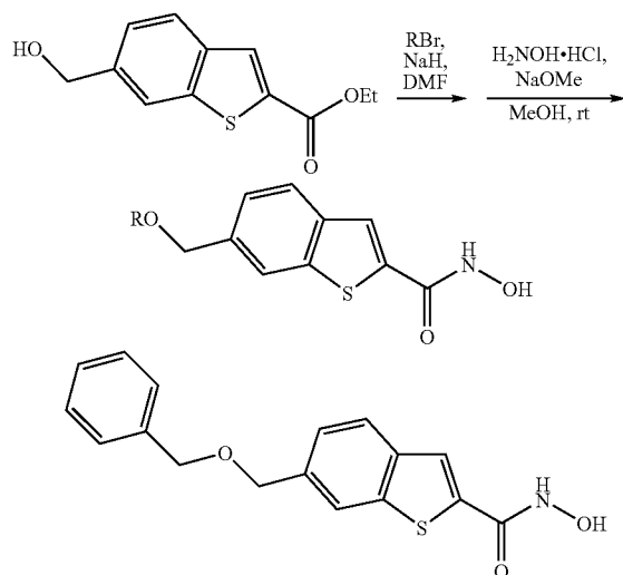
Scheme 8
