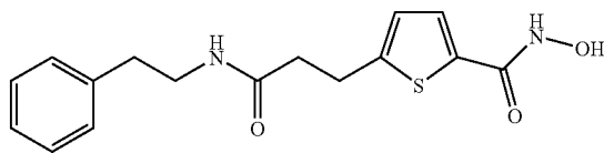
5-(2-Phenethylcarbamoyl-ethyl)-thiophene-2-carboxylic acid hydroxyamide
