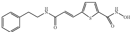
5-(2-Phenethylcarbamoyl-vinyl)-thiophene-2-carboxylic acid hydroxyamide
