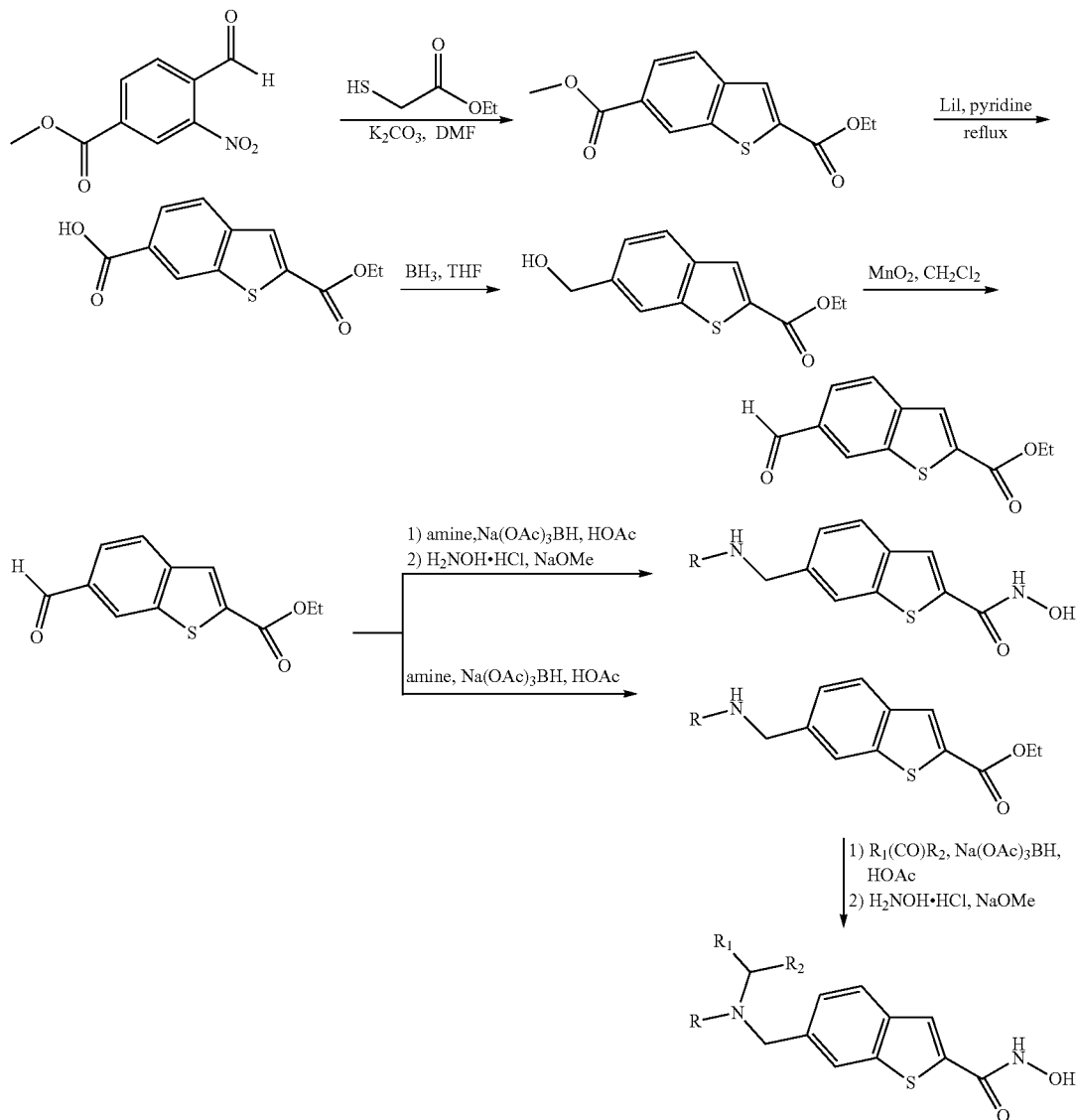
Scheme 7
