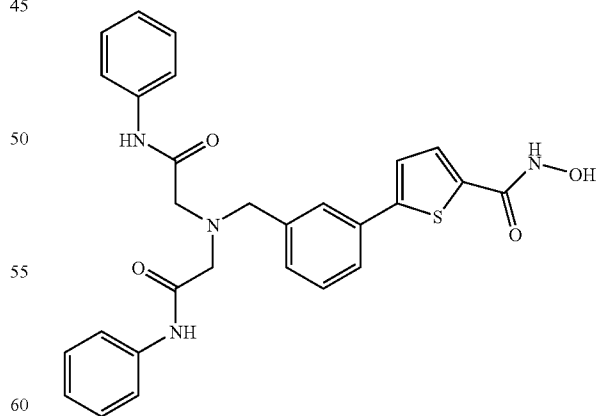
5-{3-[(Bis-phenylcarbamoylmethyl-amino)-methyl]-phenyl}-thiophene-2-carboxylic acid hydroxyamide
