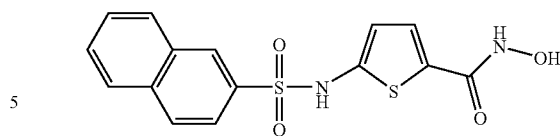
5-(Naphthalene-2-sulfonylamino)-thiophene-2-carboxylic acid hydroxyamide
