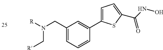
N,N-Dialkyl-5-(3-Aminomethyl-phenyl)-thiophene-2-carboxylic acid hydroxyamide
