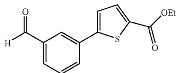
5-(3-Formyl-phenyl)-thiophene-2-carboxylic acid ethyl ester
