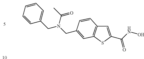
6-[(Acetyl-benzyl-amino)-methyl]-benzo[b] thiophene-2-carboxylic acid hydroxyamide
