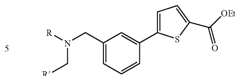
N,N-Dialkyl-5-(3-aminomethyl-phenyl)-thiophene-2-carboxylic acid ethyl ester
