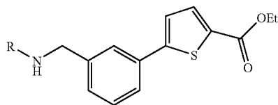
General Experimental for Amine Formation using (Formyl-Phenyl)-Thiophene
