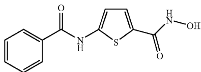
5-Benzoylamino-thiophene-2-carboxylic acid hydroxyamide
