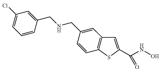
5-[(3-Chloro-benzylamino)-methyl]-benzo[b]thiophene-2-carboxylic acid hydroxyamide
