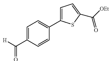
5-(4-Formyl-phenyl)-thiophene-2-carboxylic acid ethyl ester
