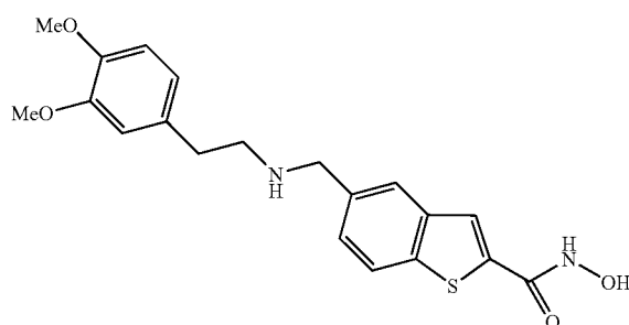
5-[(2-(3,4-Dimethoxy-phenyl)-ethylamino)-methyl]-benzo[b]thiophene-2-carboxylic acid hydroxyamide
