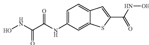
N-Hydroxy-N'-(2-hydroxycarbamoyl-benzo[b]thiophene-6-yl)-oxalamide
