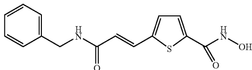
5-(2-Benzylcarbamoyl-vinyl)-thiophene-2-carboxylic acid hydroxyamide
