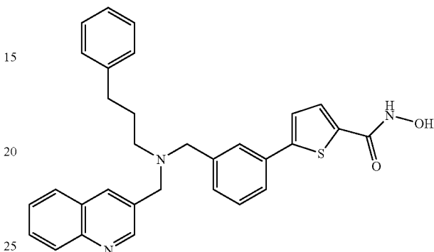
5-(3-{[(3-Phenyl-propyl)-quinolin-3-ylmethyl-amino]-methyl}-phenyl)-thiophene-2-carboxylic acid hydroxyamide
