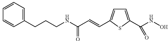
5-[2-(3-Phenyl-propylcarbamoyl)-vinyl]-thiophene-2-carboxylic acid hydroxyamide
