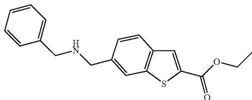
6-(Benzylamino-methyl)-benzo[b]thiophene-2-carboxylic acid ethyl ester
