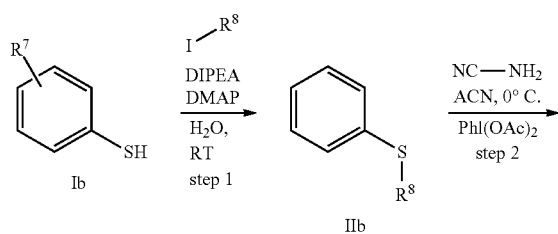
Scheme 13: Synthesis of Sulfoximine intermediate
