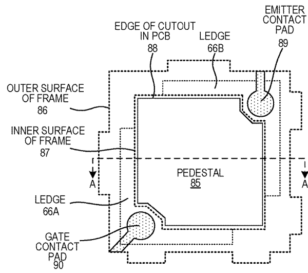
PEDESTAL LOCATION WITHIN FRAME (TOP-DOWN VIEW)
