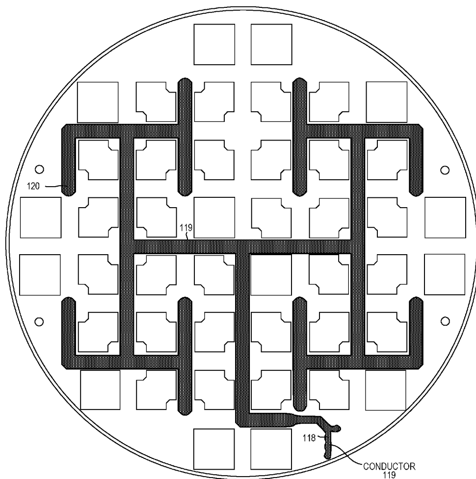
METAL LAYER 2 OF PCB FIG. 14
