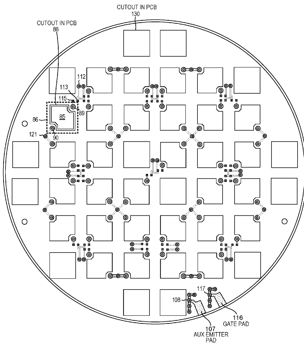
TOP METAL LAYER OF PCB
