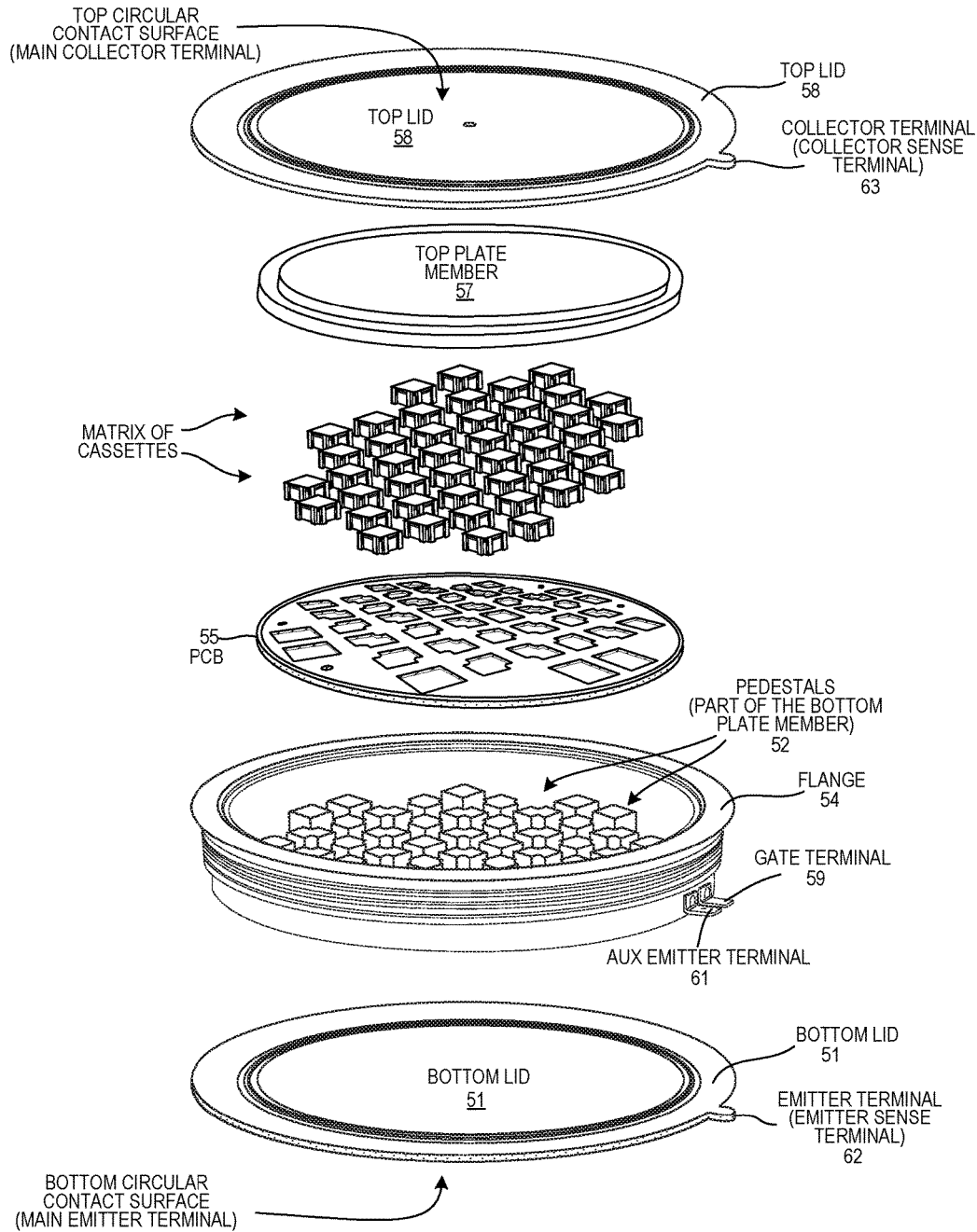
PRESS PACK MODULE ASSEMBLY (EXPLODED VIEW)
