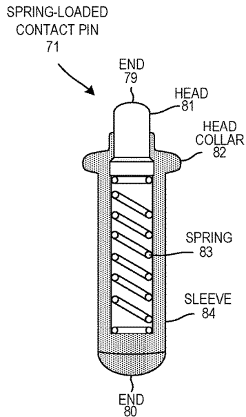
SPRING-LOADED CONTACT PIN
