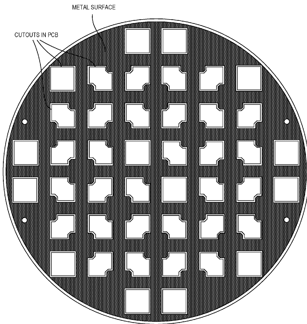
BOTTOM METAL LAYER OF PCB
