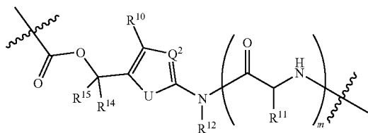
Formula (III-b)
