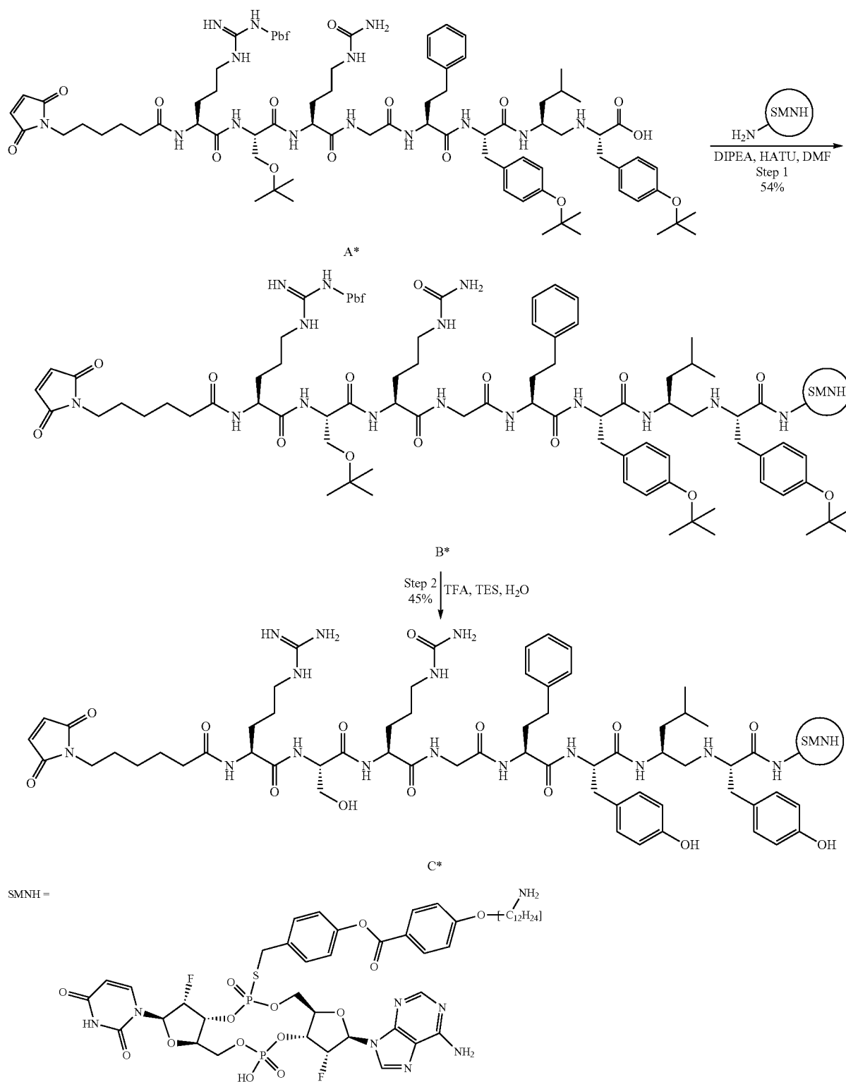
Scheme 1: Synthesis of C*
