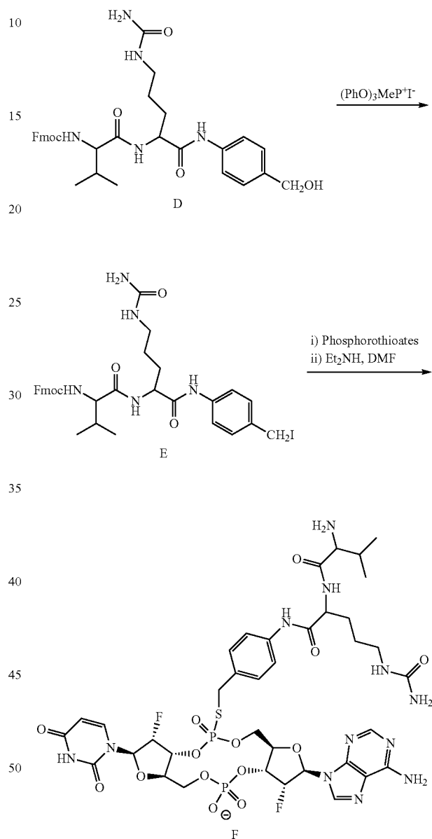
Scheme 2: Preparation of Peptide linked Phosphorothioate
