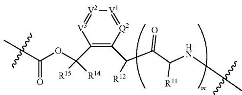
Formula (III-c)
