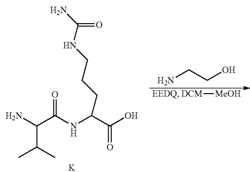
Scheme 4: Exemplary synthesis of compounds N, O, and Q.
