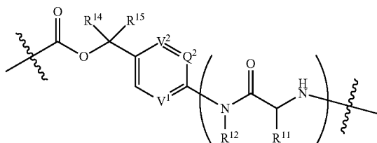
Formula (III-c)
