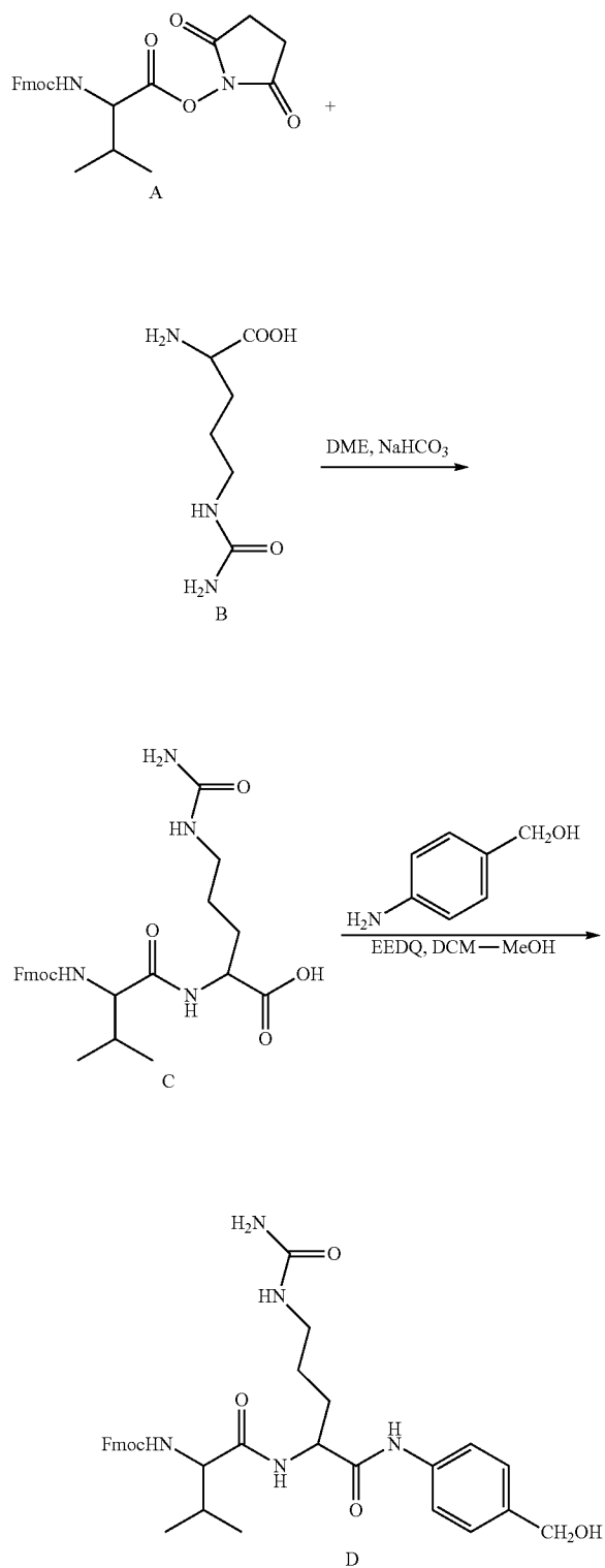
Scheme 1: Synthesis of D
